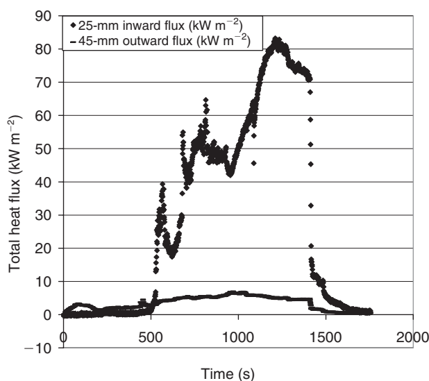
Fig. 3. Measured heat fluxes underneath and outside the burning Class B brand.
