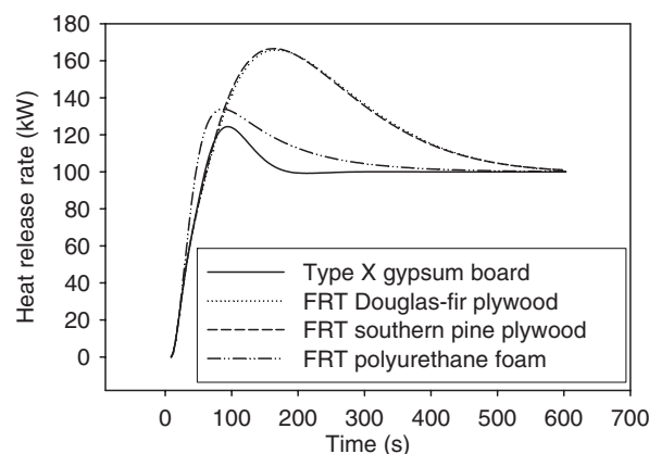
Fig. 12. Prediction of heat-release rate (HRR) for upward corner-wall flame spread on different FRT (fire retardant-treated) materials subjected to 100-kW burner (note: close agreement with room-corner test result was obtained).
