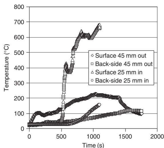
Fig. 4. Analytical prediction of dried redwood response to Class B brand heat exposure.
