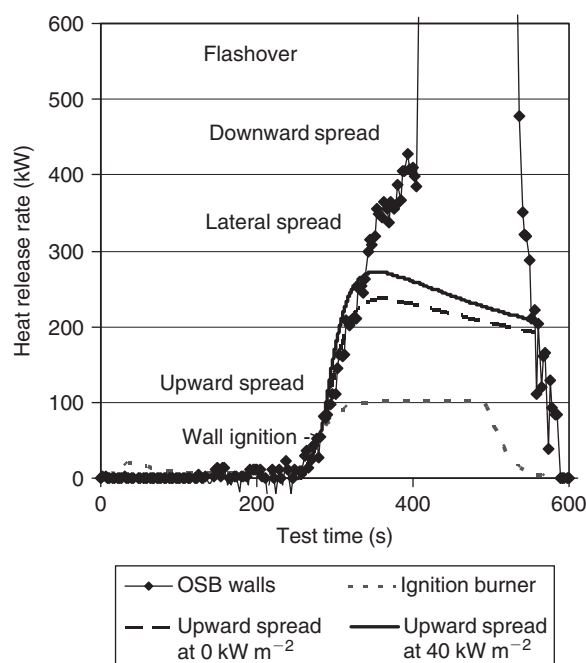
Fig. 10. Analytical prediction and room-corner test for oriented-strand board (OSB) on the walls varying the external radiant flux from 0 to 40 \text{ kW m}^{-2} .
