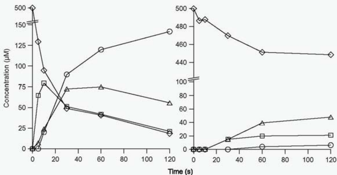
Fig. 1. Time course of AaeAPO -catalyzed oxidation of toluene (left) and 4-nitrotoluene (right). Toluenes (◇), benzylic alcohols (□), benzaldehydes (Δ), benzoic acids (○).
