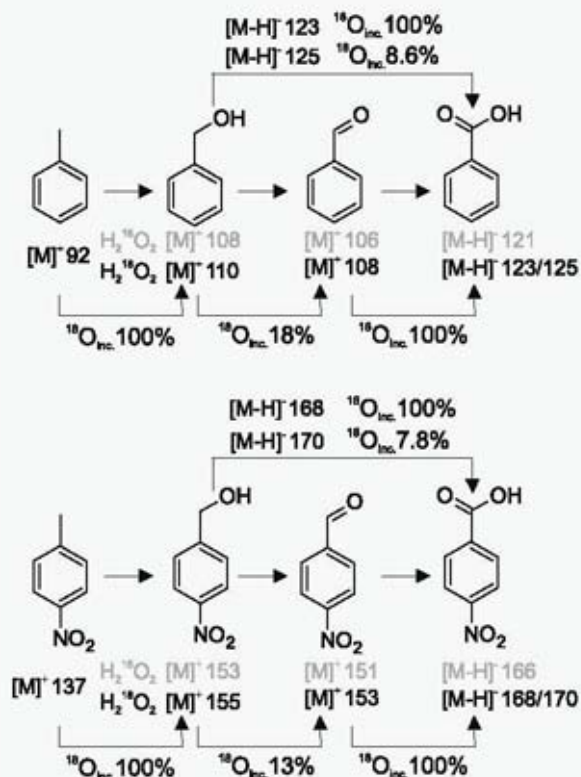
Fig. 2. Reaction scheme showing the yields of ^{18}\text{O} -incorporation into reaction products during AaeAPO -catalyzed oxidation of toluene (top) and 4-nitrotoluene (bottom) in the presence of \text{H}_2^{18}\text{O}_2 .
