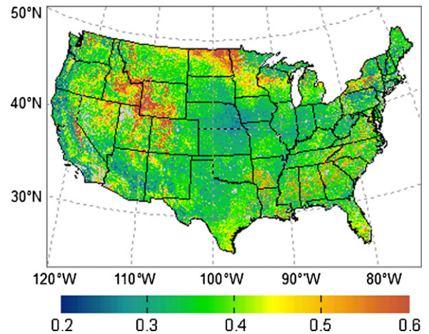
Fig. 3. Representativeness of the AmeriFlux network measured by the similarity between each grid cell and eddy flux sites using the Euclidean distance in the attribute space. The similarity is proportional to the magnitude of the distance.
