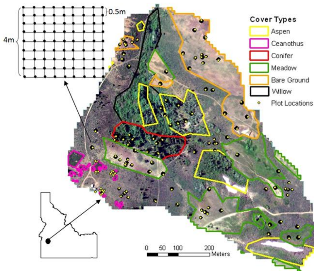
Figure 1. Cover type map of Reynolds Creek Mountain East, defined by seven classes (Willow, Ceanothus, Shrub, Bare Ground, Conifer, Meadow, and Aspen). The shrub cover type represents all areas not outlined by other cover types and the willow cover type was excluded from surveying due to the impracticality of operating equipment in saturated areas. Each set of yellow points represents the location of a 4 m by 4 m plot with survey points systematically gridded every 0.5 m (81 points/plot; 9 points/m 2 ; see inset).
