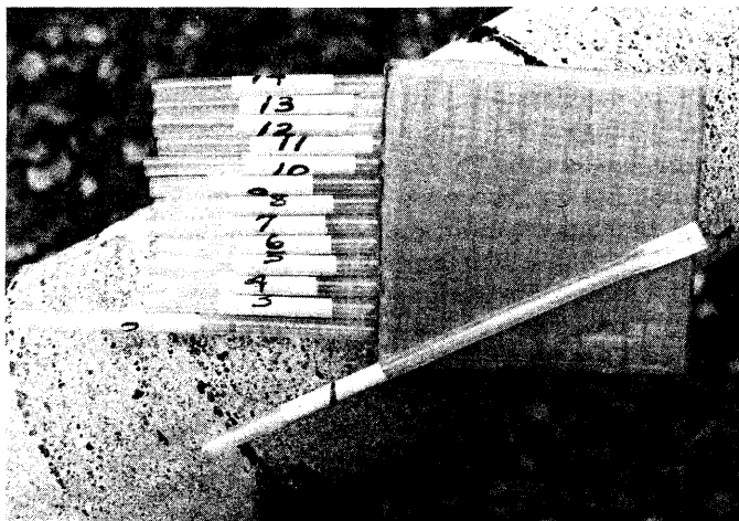
Figure 1.—Increment core carrier constructed from readily available materials.
