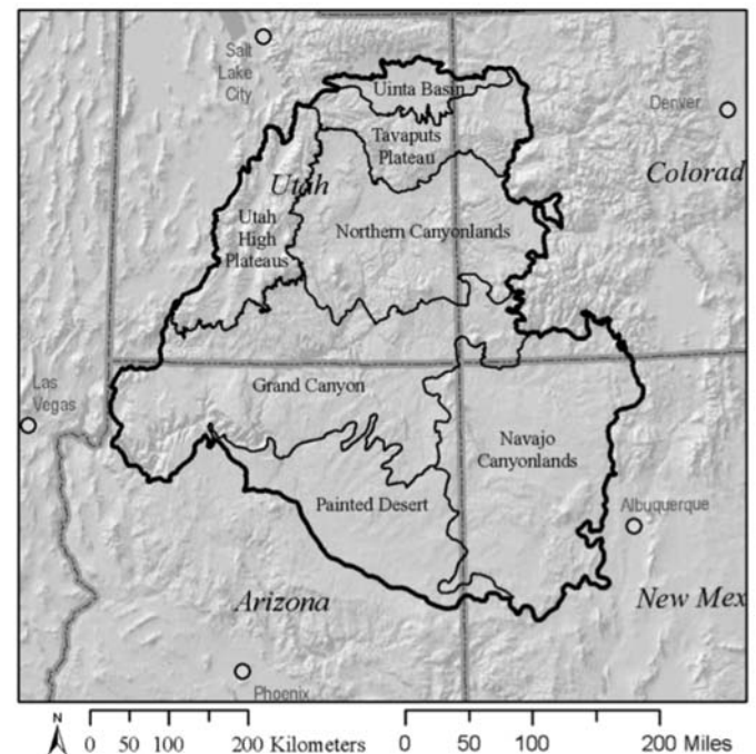
Figure 3. Ecological Sections within the Colorado Plateau.
