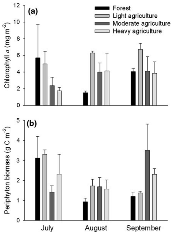
Fig. 2 Monthly mean ( \pm SE) chlorophyll a (a) and periphyton biomass (b) from rocks collected from replicate streams in each land-use type during July, August, and September
