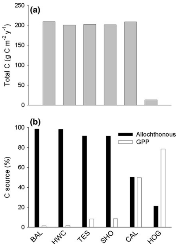
Fig. 3 Total carbon supply (a) and percentage carbon source (b) to study streams. Total carbon inputs is the sum of annual allochthonous input and GPP. In b, allochthonous origin consists of total annual litterfall ( filled bar ) and autochthonous origin includes in stream gross primary production ( unfilled bar ). BAL and HWC are forested streams, TES is a light-agriculture stream, SHO is a moderate-agriculture stream, and CAL and HOG are heavy-agriculture streams
