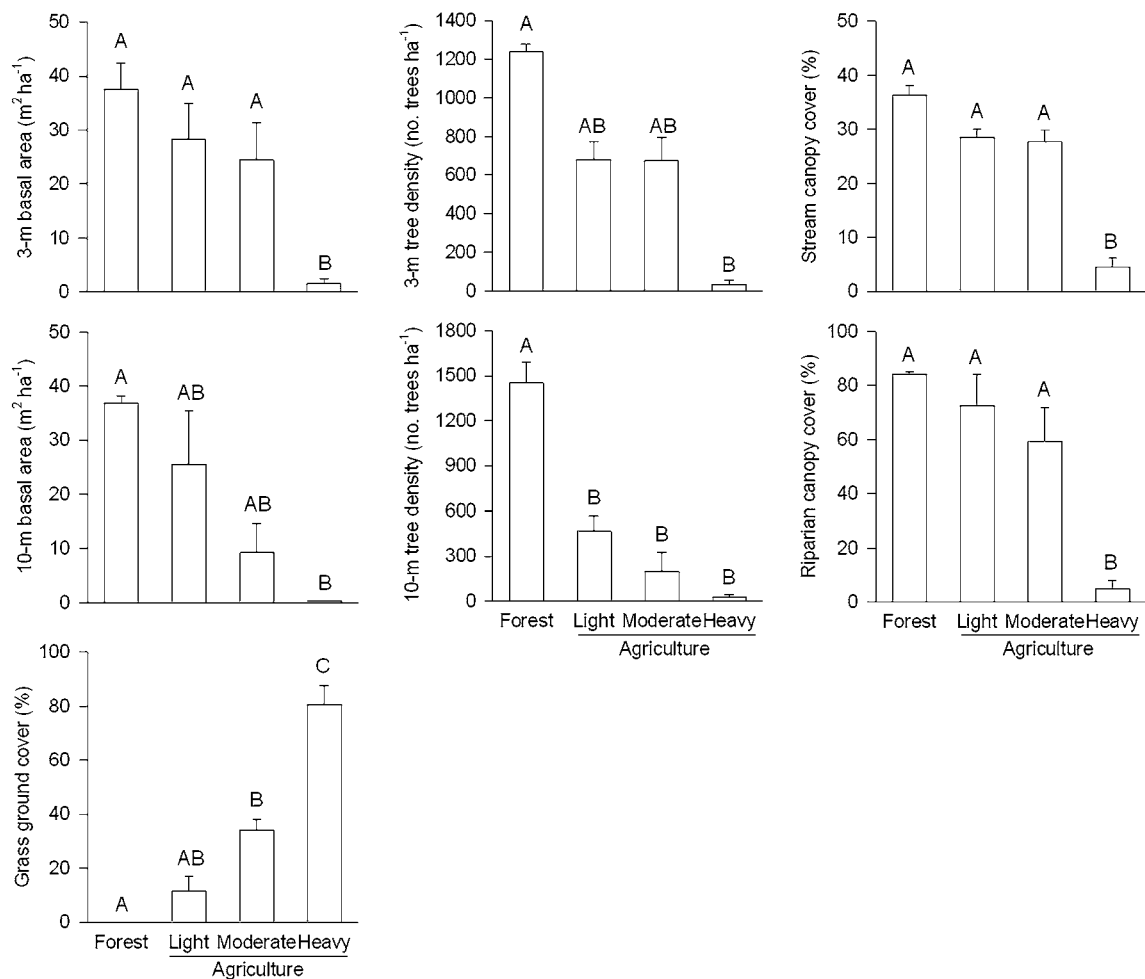
Fig. 1 Mean ( \pm SE) riparian vegetation basal area and tree density within 3 and 10 m of each stream reach, stream canopy cover along each 100-m stream reach, riparian canopy cover within 10-m of each stream reach and grass groundcover within 10-m of each stream reach for each land-use category (forested
