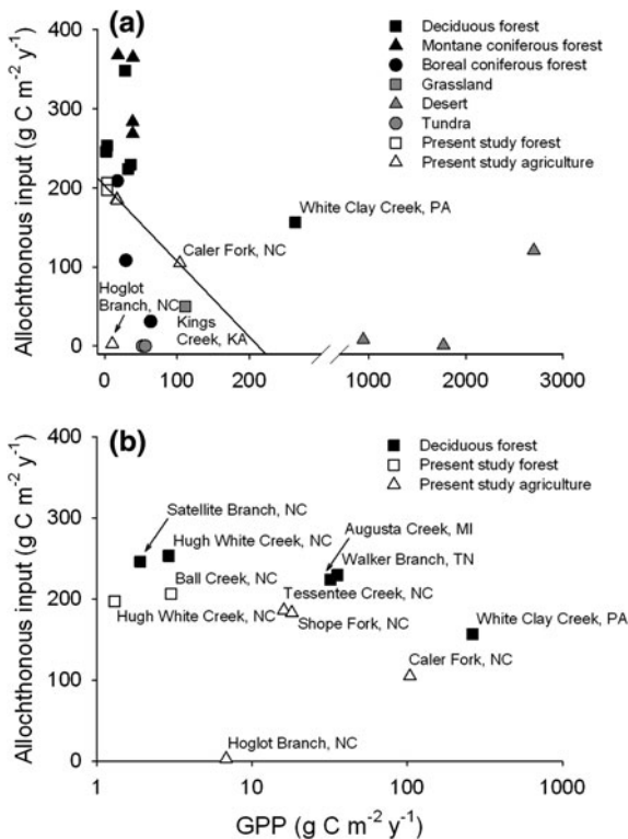
Fig. 5 Gross primary production and annual allochthonous input to streams with multiple biomes (a) and in deciduous forests (b). Data are reproduced with permission from Webster & Meyer (1997). The line in a is a linear regression extended to the axes for the streams in our study for which we have measurements of both allochthonous and autochthonous inputs with exception of Hoglot Branch ( R^2 = 0.99 )
