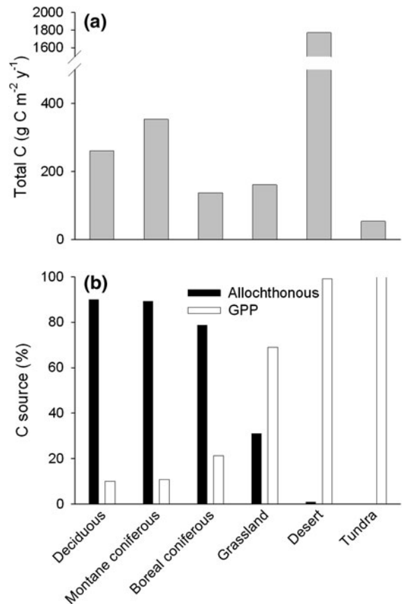
Fig. 4 Total carbon supply (a) and percentage carbon sources (b) to streams across multiple biomes. In b, allochthonous origin ( filled bar ) represents median total annual litterfall and GPP ( unfilled bar ) shows median GPP to streams in each biome. Data include 19 streams of similar size to our study streams (from Webster & Meyer 1997)
