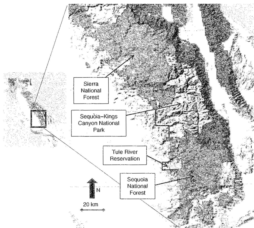
Fig. 1. Study area in the southern Sierra Nevada of California. Solid black lines designate western boundaries of Sequoia-Kings Canyon National Park and Tule River Reservation.
