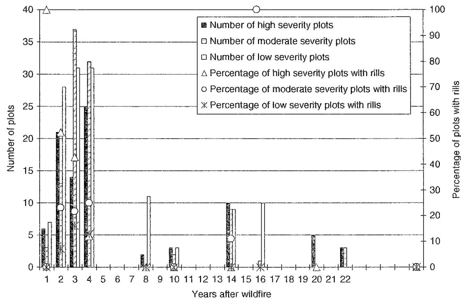
Fig. 3. Number of wildfire plots by years since burning and wildfire severity and percentage of rilled plots by severity and years after burning.
