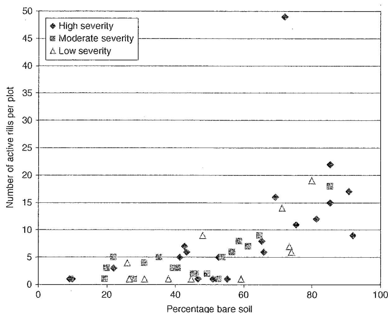
Fig. 5. Active rill frequency v. percentage bare soil and wildfire severity.
