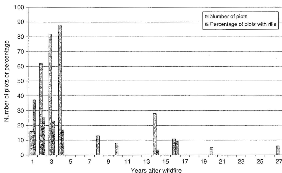
Fig. 2. Number of wildfire plots by years since burning and percentage of plots with rills.
