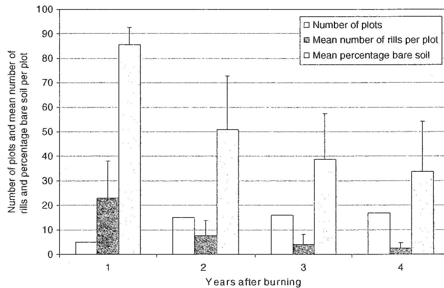
Fig. 4. Mean and standard deviation of rills and percentage bare soil per plot for plots surveyed in multiple years, for the first 4 years after wildfire. Five rills at 14 years and two rills at 16 years are not shown.
