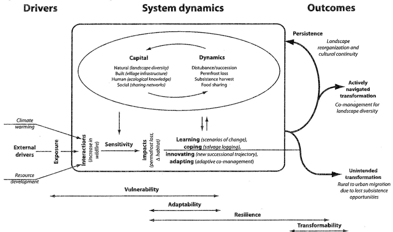
Fig. 2. System perspective on the vulnerability and resilience of the Alaskan boreal forest, showing how changes in drivers (left side) modify the system to produce resilient or transformational outcomes (right side). The arrows at the bottom show the range of processes associated with vulnerability, adaptability, resilience, and transformability. Multiple external stresses (climate warming and resource development) interact to increase the extent and severity of wildfire. This, in turn, creates impacts (permafrost loss and habitat change). Social learning (learning, coping, innovating, and adapting) in response to these impacts has the potential to alter social–ecological interactions and various forms of capital of the system, which in turn, influence sensitivity to future events. Social learning also governs the relative likelihood of three potential outcomes: persistence of the existing system through resilience; actively navigated transformation to a new, potentially more beneficial trajectory through transformation; or unintended degradation to a new state due to vulnerability and failure to adapt or transform. Modified from Chapin et al. (2009a).
