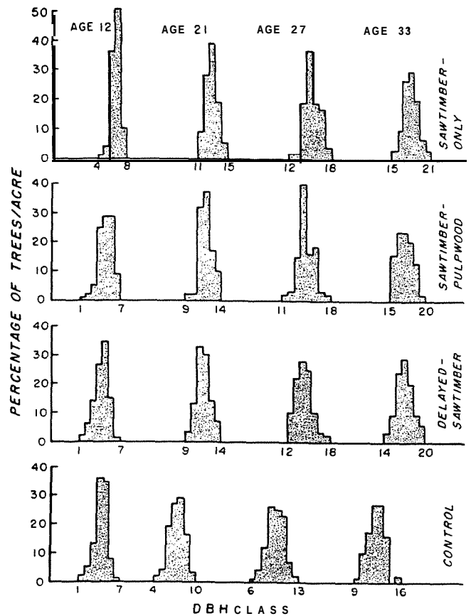
Figure 4.—Stand structure by treatment before thinning at ages 12, 21, 27, and 33.
