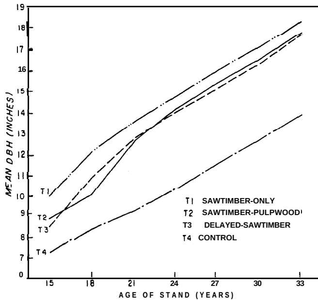
Figure 3.—Quadratic mean dbh by treatment and age of the 48 largest trees per acre (36 trees at age 33).
