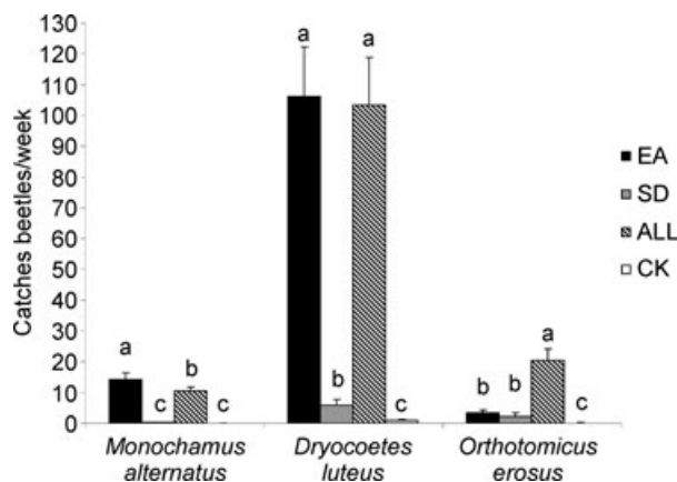
Fig. 1 Catches of M. alternatus , D. luteus and O. erosus in unbailed traps (CK) and traps baited with ethanol and (+)- \alpha -pinene (EA), ipsenol and ipsdienol (SD), ethanol, (+)- \alpha -pinene, ipsenol and ipsdienol (ALL) ( n = 10 ). For each species, means followed by a different letter are significantly different at \alpha = 0.05 using the Bonferroni approach.
