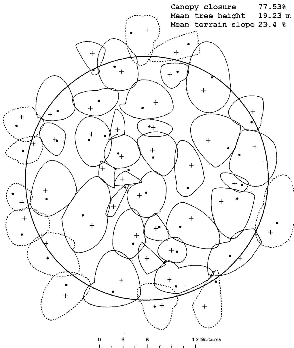
Figure 3. Field-delineated crowns, surveyed tree bases (●), and LiDAR-assessed tree tops (+) of a plot in a deciduous stand with medium canopy cover. The thick line represents the boundary of the 15-m-radius plot. Crowns of trees with base outside of the plot are represented with dashed lines.
