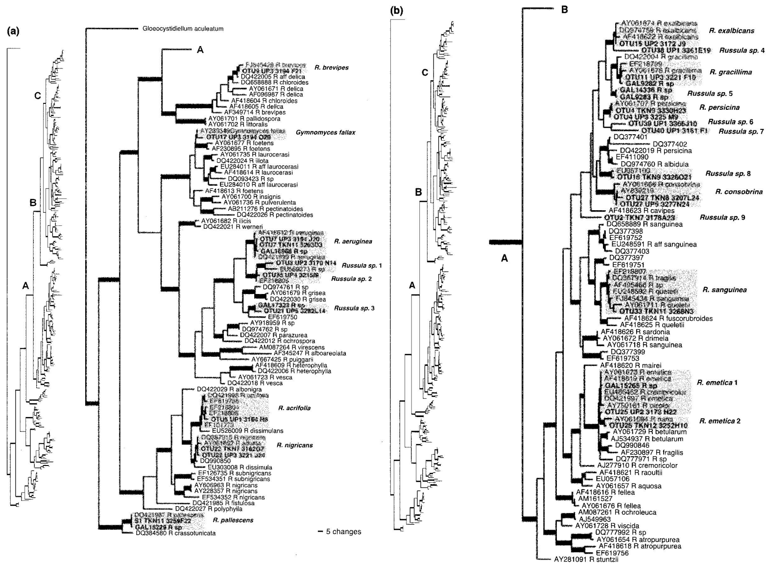
Fig. 2 Maximum-likelihood phylogram ( \text{Log}_e = 29\ 146.2106 ) inferred from the internal transcribed spacer (ITS) rDNA dataset showing the phylogenetic spread of boreal Alaskan Russula soil clone operational taxonomic units (OTUs) and sporocarp sequences (bold text) generated in this study among representatives of Russula taxa in GenBank. Sequences with GAL numbers were derived from herbarium specimens, whereas OTUs of UP and TKN sequences in bold are from soil clone libraries of upland mixed forest and lowland black spruce forest, respectively. Branches with Bayesian posterior probability support \geq 0.95 are thickened. Phylogroups including Alaskan sequences are indicated by gray boxes and are named following OTU identification in Table 2 or based on closest relatives. GenBank sequences with no name attached are from unidentified environmental samples. Clades marked by 'A', 'B' and 'C' are shown in detail in parts (b), (c) and (d), respectively.
