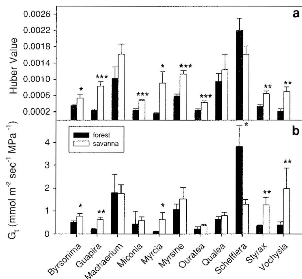
Fig. 2 a Huber value (sapwood area:leaf area) and b apparent leaf-area specific hydraulic conductance of the soil/root/leaf pathway ( G_t ) of savanna and forest congeneric species. Error bars represent SEs. * P \leq 0.05 , ** P \leq 0.01 , *** P \leq 0.001
