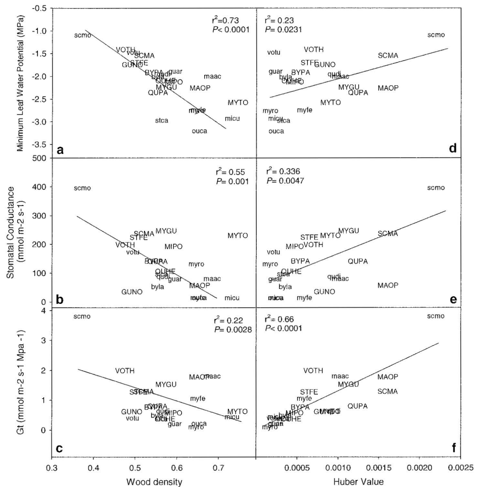
Fig. 3 Correlations between dry season leaf water potential, stomatal conductance, G_i and wood density (a–c), or Huber value (d–f). For all correlations the line represents the linear regression between the two variables. The slopes of the trait relationships for savanna and forest trees did not significantly differ from one another, thus, relationships are shown using a single regression line. Abbreviations comprise the first two letters of the genus name followed by the first two letters of the specific epithet (see Table 1 for full names): four-letter uppercase codes indicate savanna species, four-letter lowercase codes indicate forest species
