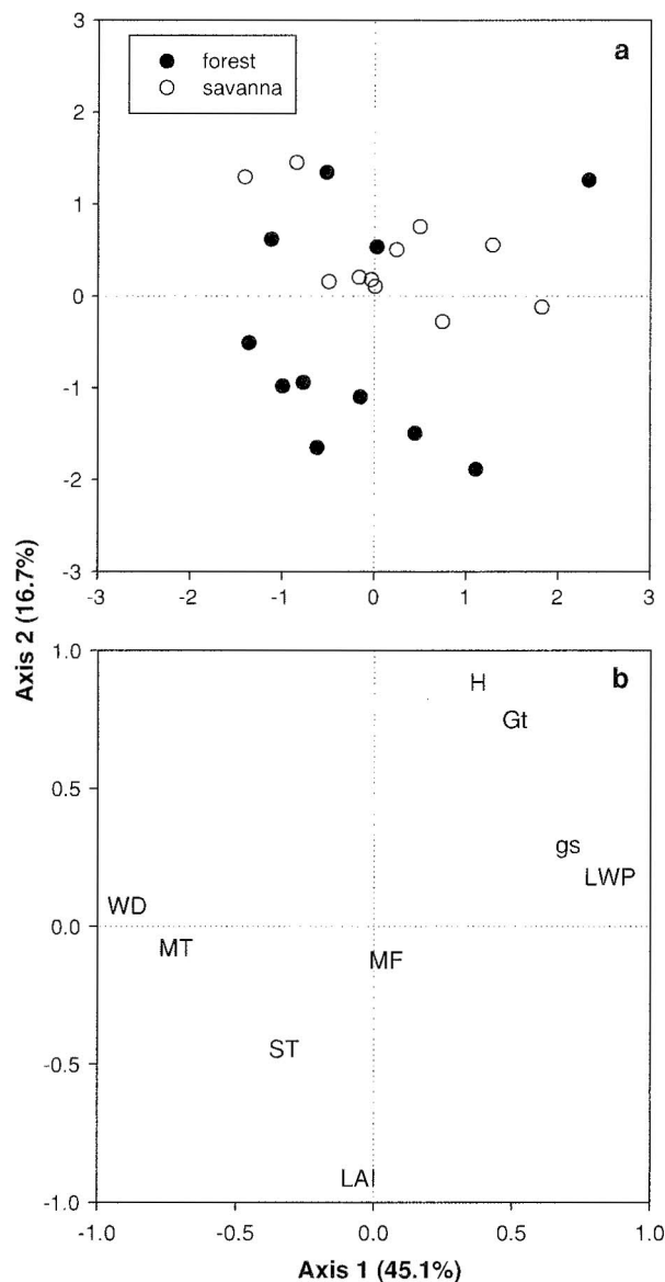
Fig. 4 Position of forest and savanna species (a) and traits (b) on the first two axis of the principal components analysis for all the traits included in this study. Both forest and savanna species were spread evenly along the first axis, while these groups were separated along the second axis. For abbreviations, see Table 2
