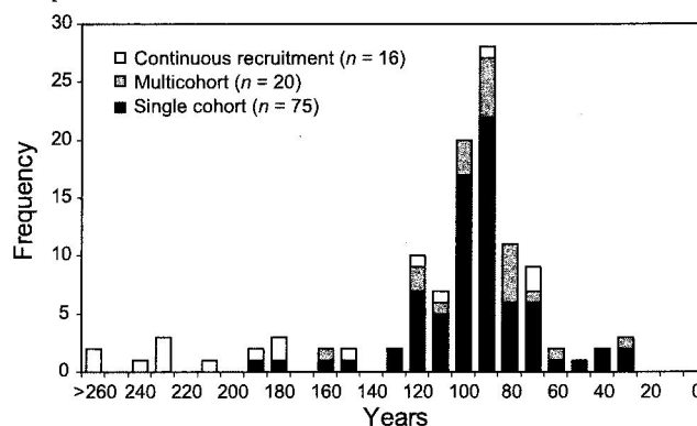
Fig. 1. Frequency histogram of prefire stand ages (in years) from stands of black spruce that burned in 1994 ( n = 21 stands in one fire; Johnstone and Kasischke 2005) or 2004 ( n = 90 stands in three fires; Johnstone et al. 2010). Stand ages were estimated from tree-ring counts sampled near the tree base from trees that were alive when the stand burned ( n = 5-10 trees/stand). Most stands showed an age structure indicative of a single cohort (black bars) or two cohorts (grey bars) of trees, as tree ages clustered closely into one or two groups, respectively. We assumed the youngest cohort represented the most recent cycle of postfire recruitment and estimated the age of these stands as the age of the oldest tree in the youngest cohort. Stands that showed no clustering of tree ages appeared to have experienced continuous recruitment since the last fire (white bars), and stand age was estimated from the oldest sampled tree.
