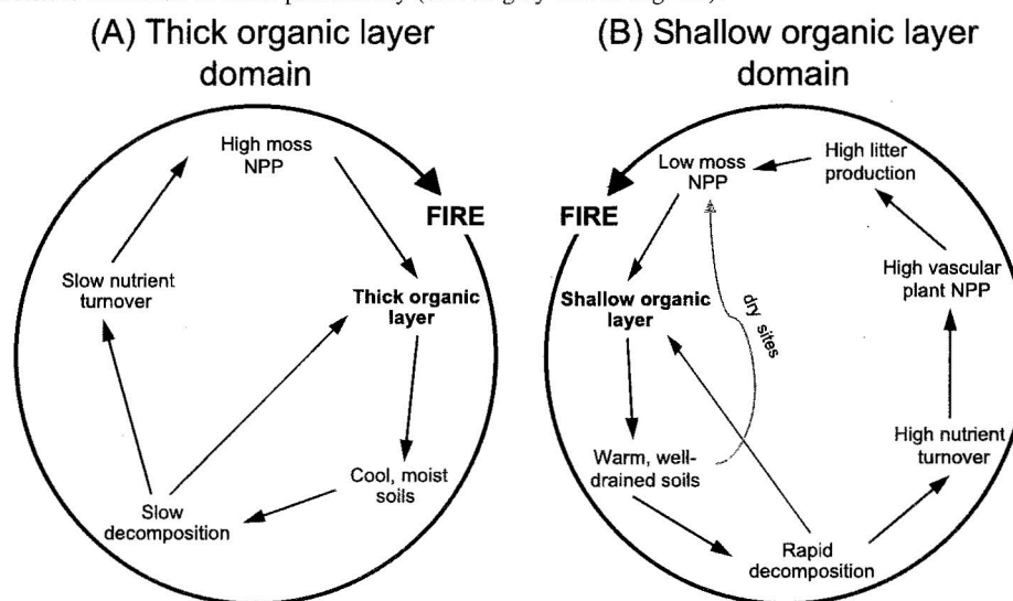
Fig. 2. Soil organic layer dynamics across fire and successional cycles representing alternative stability domains. In the thick organic layer domain (A), the accumulation of soil organic layers in mesic-to-moist sites is associated with feedbacks among cool, moist soils; low rates of decomposition and nutrient cycling; and high moss productivity (net primary productivity, or NPP). Alternatively in the shallow organic layer domain (B), shallow organic layers in mesic-to-dry sites are associated with feedbacks among warm, dry soils; high rates of decomposition; and high vascular plant productivity that smothers mosses with deciduous leaf fall. Shallow organic layers are also maintained at dry sites by direct moisture limitation of moss productivity (curved grey line in Fig. 2B).
