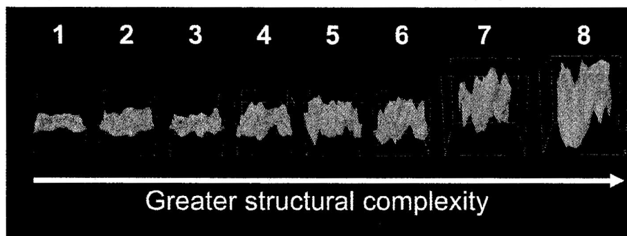
Fig. 1. Examples of the range of canopies for plots used in this study. Each canopy surface shown was created for one of the plots from the LiDAR data (30 m × 30 m areas). Canopies were considered to be more structurally complex as crown heights and rumple values increase and as canopy densities (proportion of canopy with foliage blocking view of the ground from the LiDAR instrument) decrease through the formation of gaps. Table 2 provides measured field and LiDAR metric values for these example plots.
