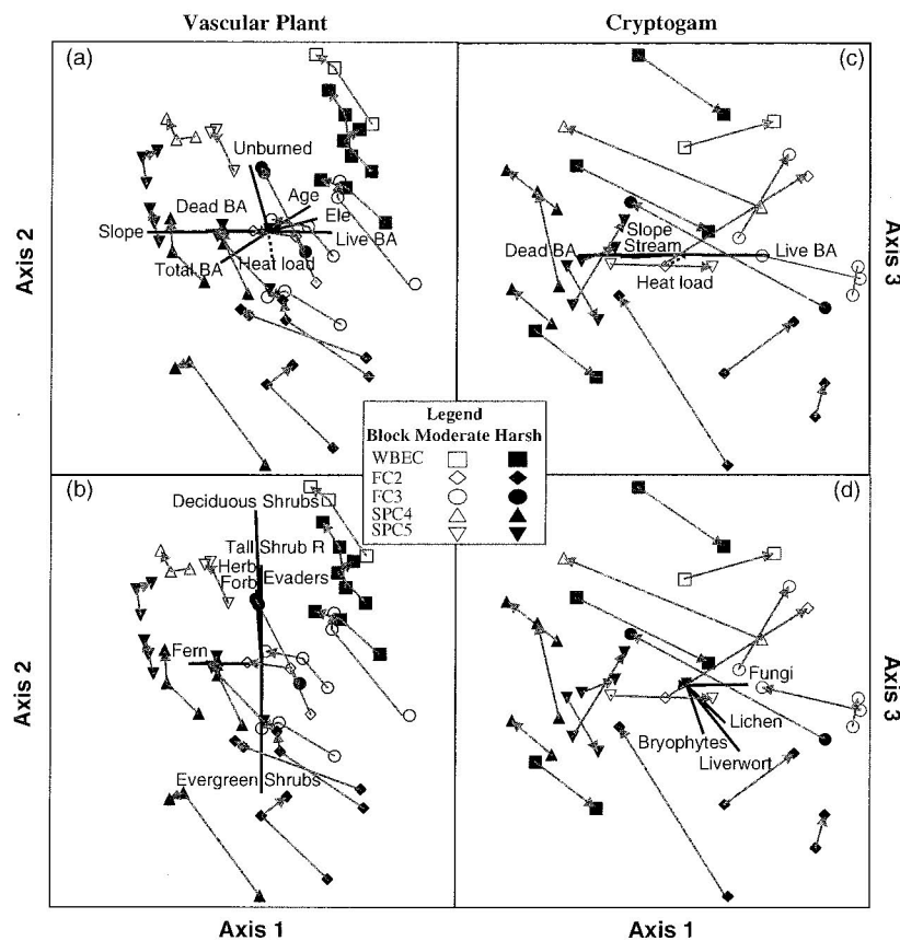
Fig. 2. Three-dimensional NMS ordinations of vascular plant (a and b: R^2 = 69\% for all three axes) and cryptogam (c and d: R^2 = 81.8\% for all three axes) post-fire communities for treatments without vegetation removal. Successional arrows (gray) connect the same plot through years. Environmental (a and c) and trait (b and d) variable joint plots are overlain. Angles and length of joint plot lines (black) represents the direction and strength of relationships with environmental variables (Moderate = moderate aspect, harsh = harsh aspect, BA = basal area, Dead BA = % dead BA, Live BA = % live BA, Ele = elevation, Age = plantation age at time of burn, R = Richness, Stream = distance to stream and Unburned = distance to unburned forest). Cryptogam community axes were rigidly rotated to align % live BA with axis 1. All correlations have R^2 \geq 0.2 except dashed lines are R^2 \geq 0.08 .
