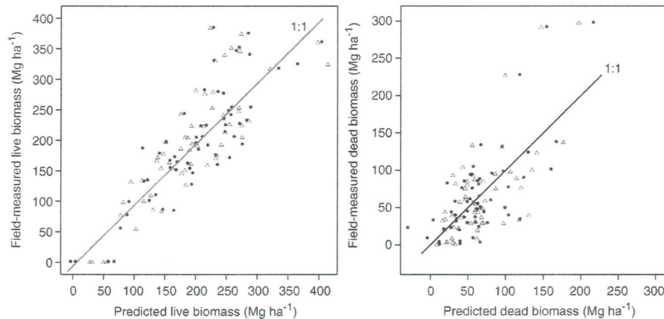
Fig. 5. Cross validation scatterplots: (left) live biomass and (right) dead biomass. Black circles are the stepwise regression models, and triangles are the alternative predictor models.
