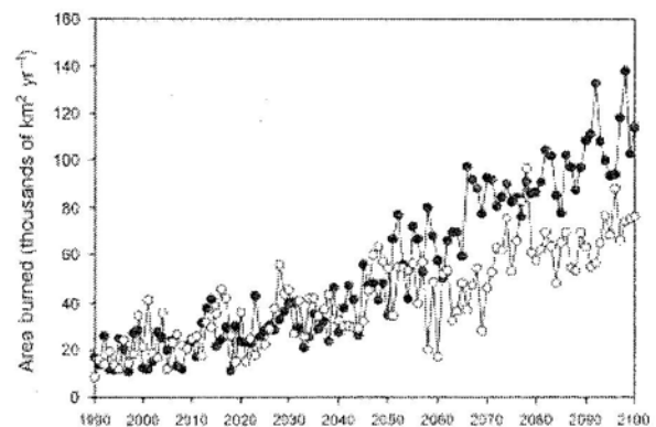
Fig. 2 Predicted annual area burned (thousands of km 2 yr -1 ) driven by using NCEP model development data sets ('Observed'; 1990–2005) and the CGCM2 A2 and B2 Scenarios (2006–2100) from Balshi et al. (2008) for Alaska and western Canada. Dark circles represent the estimates driven by the A2 scenario while the open circle represent the estimate driven by B2 scenario.
