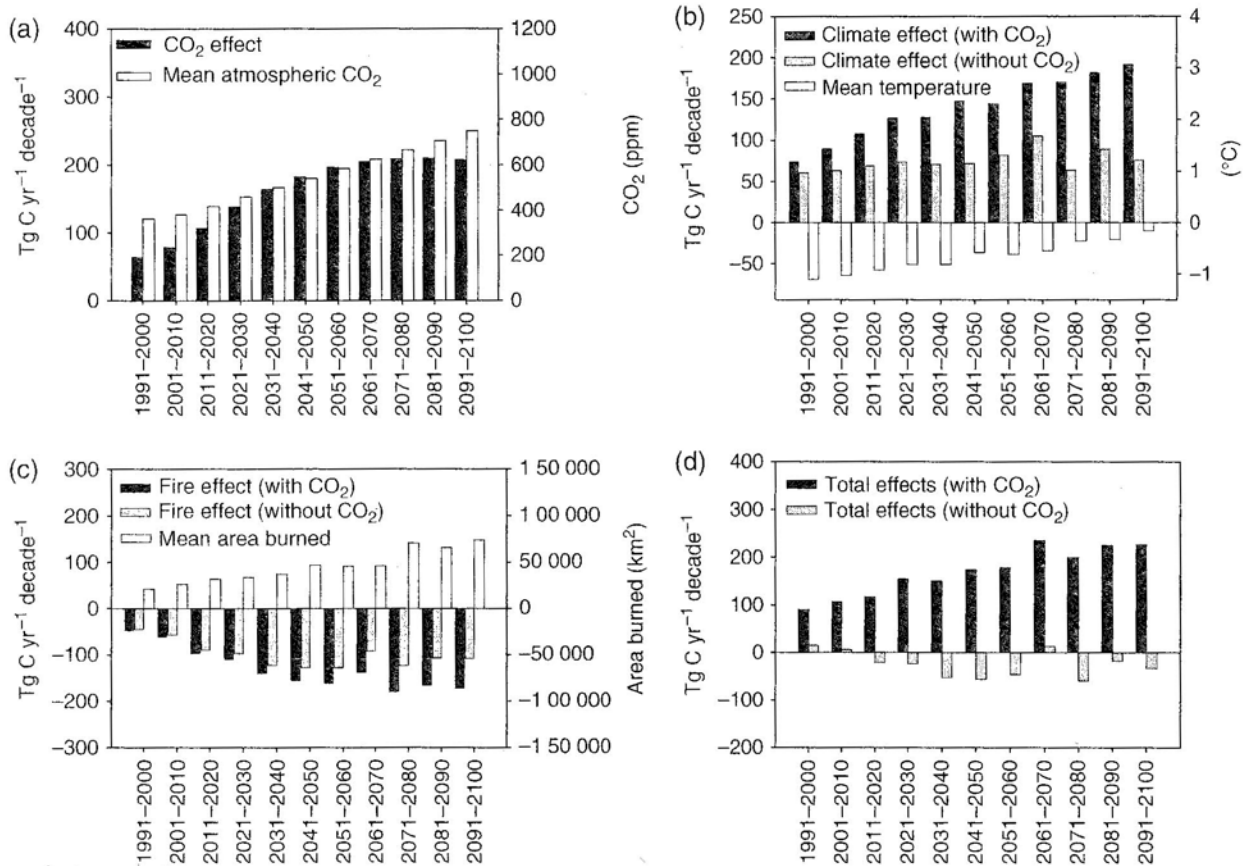
Fig. 8 Mean decadal effects from the B2 scenario simulations of (a) CO 2 , (b) climate, (c) fire, and (d) the combined effects of CO 2 , climate, and fire on simulated net ecosystem carbon balance for boreal North America for the 21st century. Also included is the last decade of the 20th century for reference. Each effect is compared with model driving data of mean decadal atmospheric CO 2 concentration, mean decadal air temperature, and mean decadal area burned across boreal North America. Positive values represent carbon sequestration by terrestrial ecosystems, while negative values represent a release of carbon from the land to the atmosphere.
