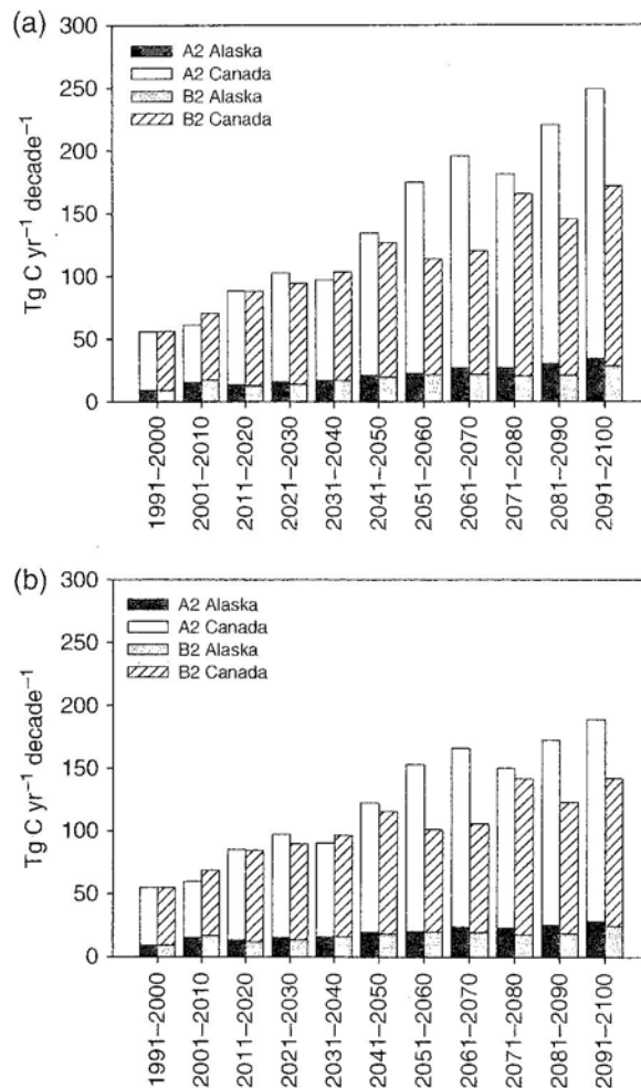
Fig. 3 Mean decadal total carbon emissions resulting from fire for boreal North America during the 21st century that (a) incorporate the effect of atmospheric \text{CO}_2 on photosynthesis and (b) exclude the role of atmospheric \text{CO}_2 fertilization on photosynthesis. The decade 1991–2000 is used as a comparison period and corresponds to years where fire emissions are driven by historical fire records. Units are \text{Tg C yr}^{-1} \text{ decade}^{-1} .
