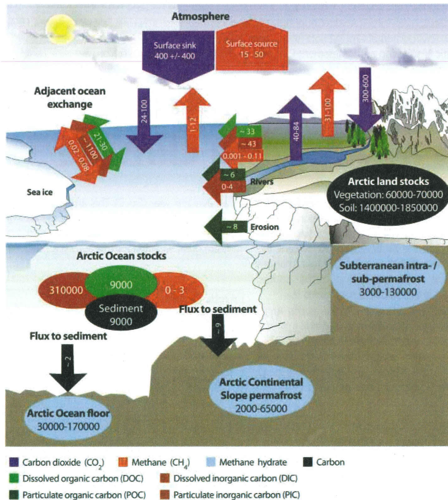
Figure 2. Current state of the Arctic carbon cycle showing amounts of carbon stored in various environmental reservoirs (units: millions of tonnes C, or millions of tonnes \text{CH}_4 for methane and methane hydrate) and the net flux of compounds (units: millions of tonnes C per year, or millions of tonnes \text{CH}_4 per year for methane) that determine the movement of carbon between environmental compartments. Source: [7].
