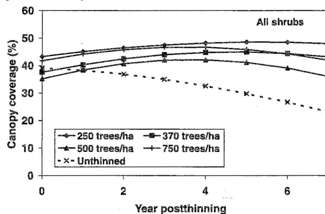
Fig. 5. Regression trend lines of total shrub canopy coverage over time. Regressions differed significantly for thinned (all four densities) versus unthinned treatments, but did not differ among thinned treatments. Pretreatment data were collected in the growing season prior to thinning.
