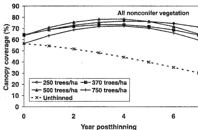
Fig. 3. Regression trend lines of total nonconifer vegetation (i.e., understory) canopy coverage over time. Regressions differed significantly for thinned (all four densities) versus unthinned treatments but did not differ among thinned treatments. Pretreatment data were collected in the growing season prior to thinning.
