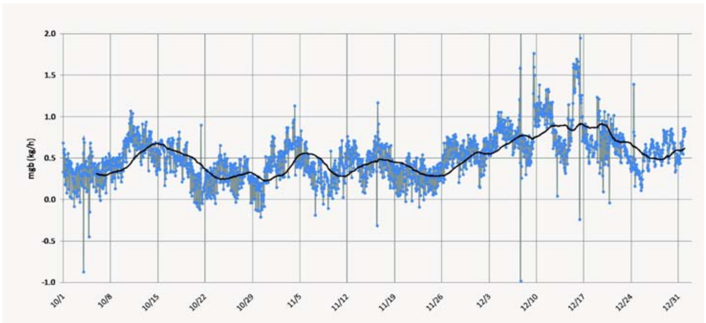
Figure 7 Moisture transport into basement (kg/h) with 5 day moving average.
