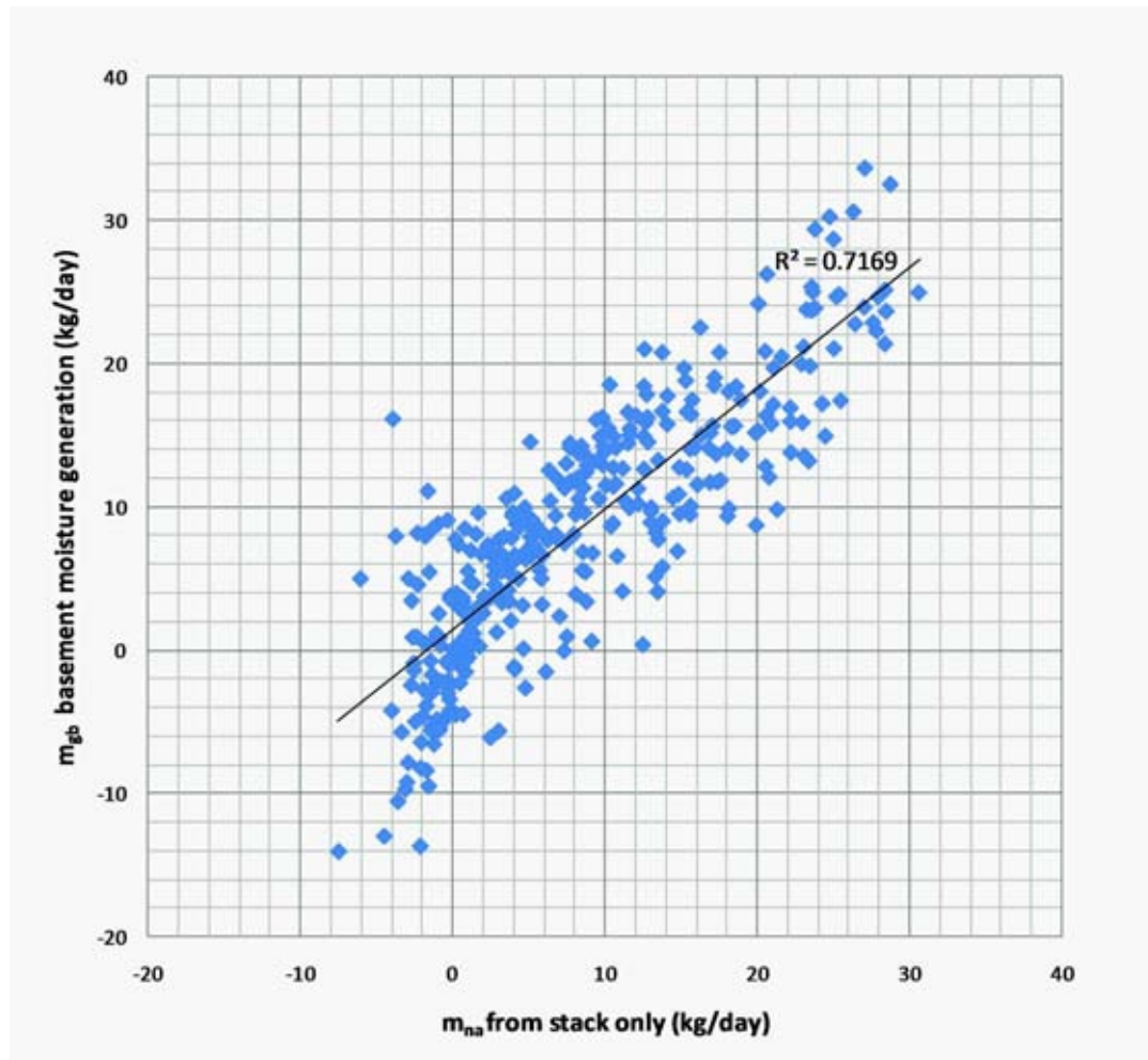
Figure 10 Correlation of total basement moisture transport with moisture loss due to stack effect.
