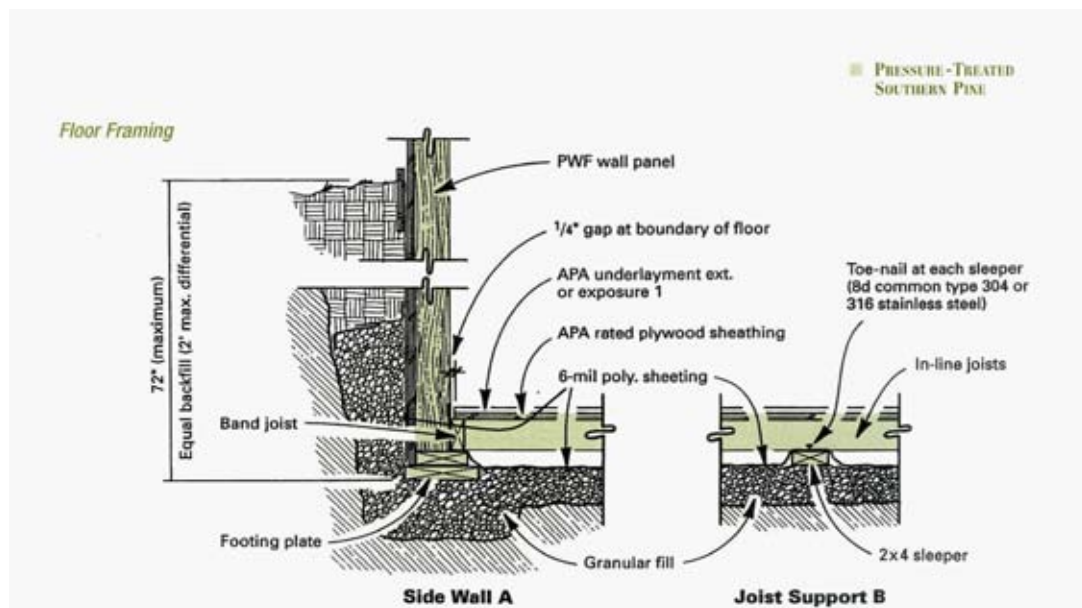
Figure 1 FPL R-Demo house basement floor and wall details.
