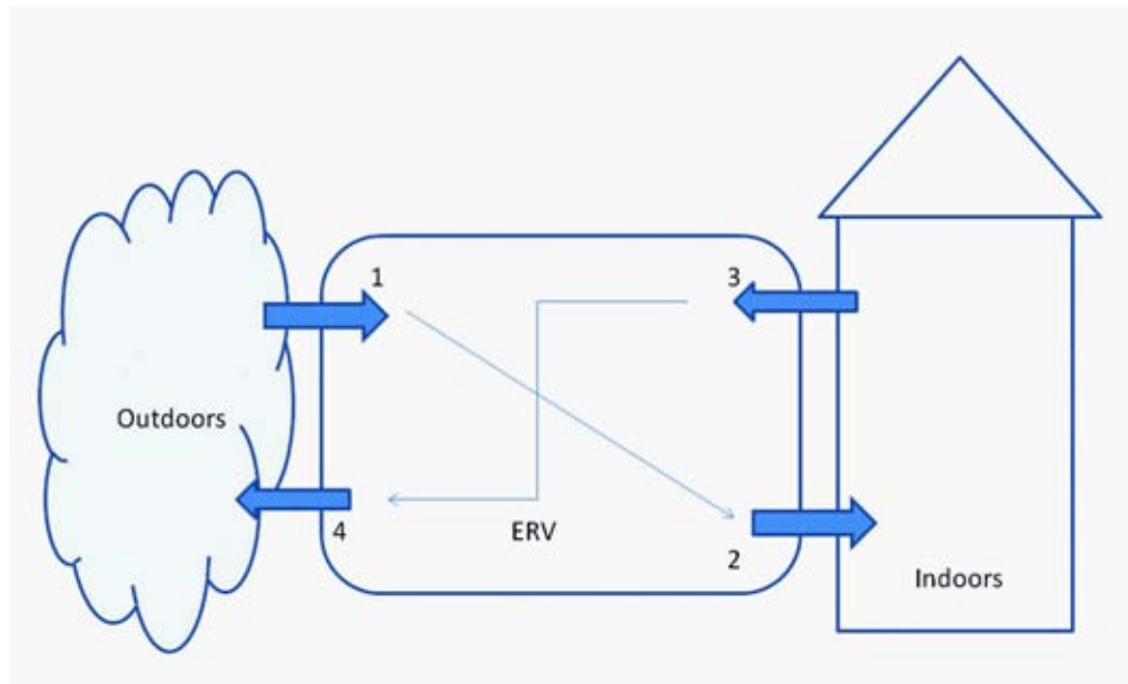
Figure 3 ERV port numbers.
