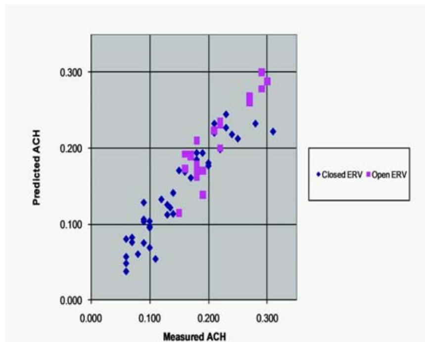
Figure 4 Predicted ach from AIM-2 versus measured ach from tracer gas study.
