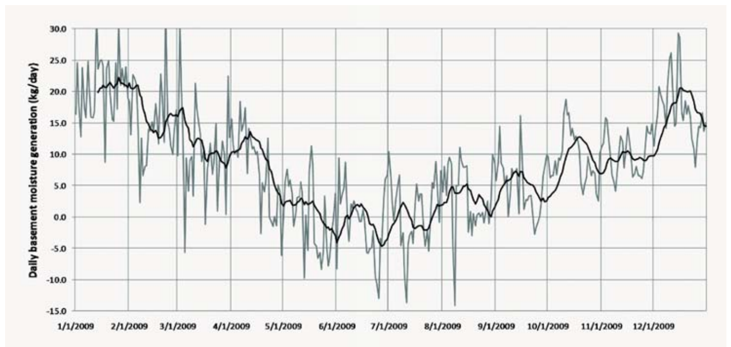
Figure 8 Moisture transport into basement (kg/day) with 14 day moving average.
