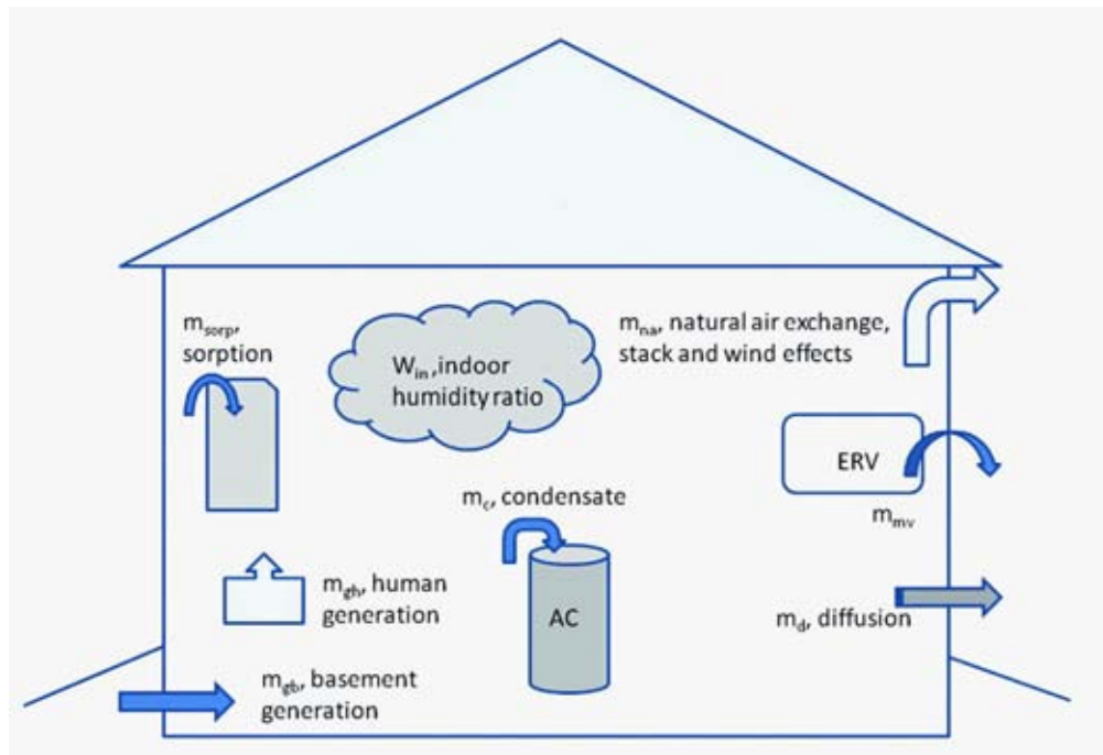
Figure 2 Moisture balance terms.
