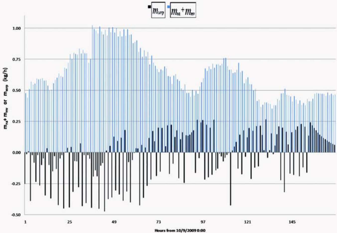
Figure 9 Hourly contributions to moisture transport by sorption and airflow.
