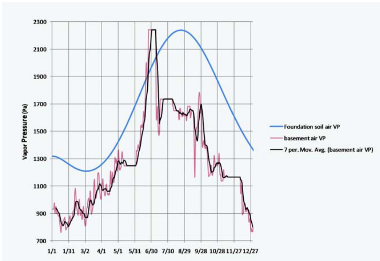
Figure 11 Vaporpressure of soil moisture and basement air
