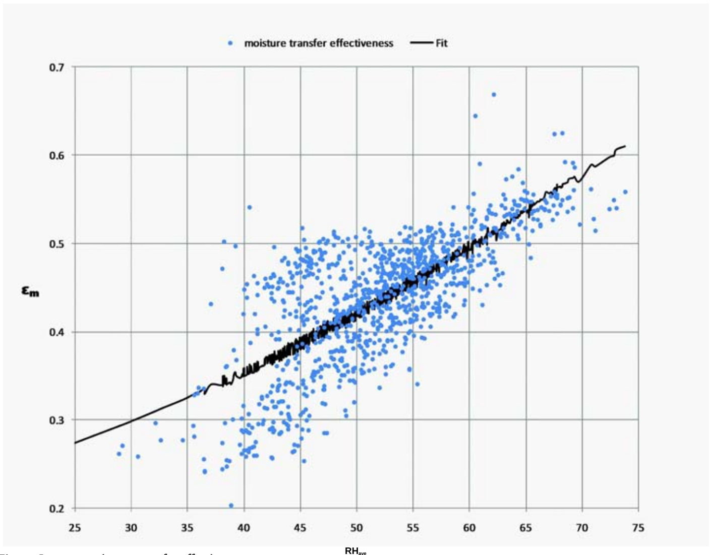
Figure 5 ERV moisture transfer effectiveness.
