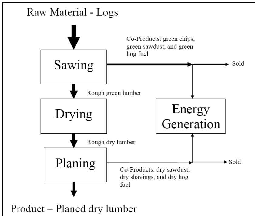
Figure 2.1 Material flow for the three unit processes of softwood lumber manufacturing.
