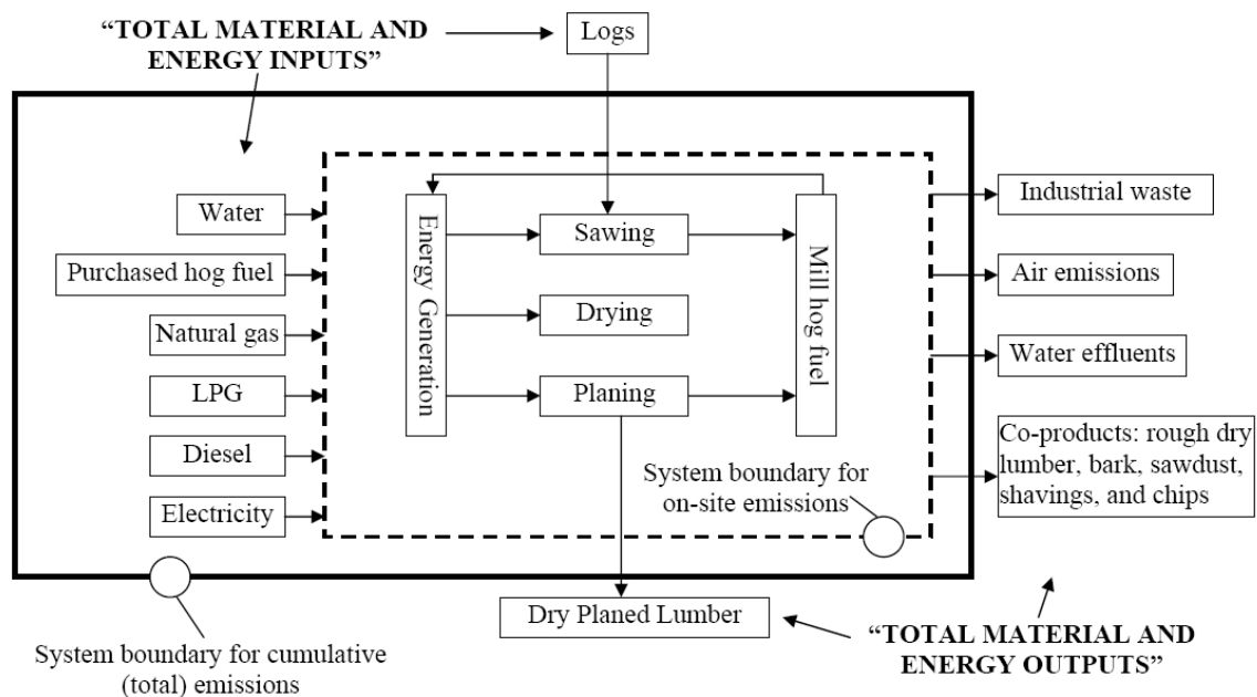
Figure 2.2 System boundaries for softwood lumber production.
