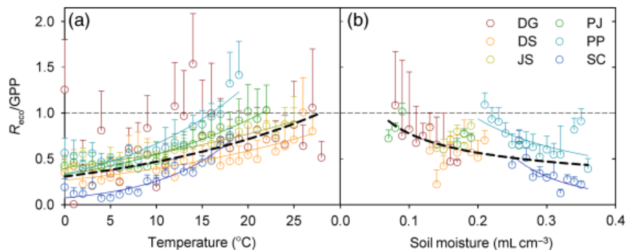
Fig. 4 Relative advantage of daily respiration over production ( R_{eco}/GPP ) as a function of (a) air temperature and (b) soil moisture (30–40 cm depth; months where low temperatures do not limit growth) for all six sites across the NMEG. Colored lines represent significant ( P < 0.05 ) within-site relationships, and dashed black lines represent the average response across sites ( P < 0.005 for both). GPP, gross primary production; R_{eco} , release through ecosystem respiration; NMEG, New Mexico Elevational Gradient; DG, desert grassland; DS, desert shrubland; JS, juniper savanna; PJ, piñon-juniper woodland; PP, ponderosa pine forest; SC, subalpine conifer forest.
