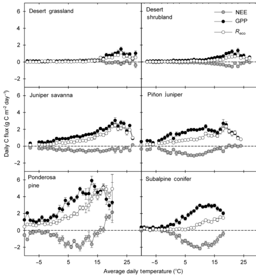
Fig. 2 Daily carbon dioxide fluxes – GPP, R_{\text{eco}} , and NEE – over the entire year as a function of mean daily temperature across the NMEG. For illustrative purposes, data are binned into 1^\circ\text{C} intervals. Plotted are the mean \pm 1 SE for each bin. GPP, gross primary production; R_{\text{eco}} , release through ecosystem respiration; NEE, net ecosystem exchange; NMEG, New Mexico Elevational Gradient.
