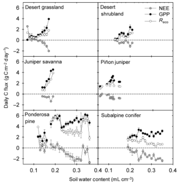
Fig. 3 Daily carbon dioxide fluxes – GPP, R_{eco} , and NEE – as a function of mean daily soil water content (30–40 cm depth) during periods when growth is not inhibited by low temperatures for all six sites across the NMEG. For illustrative purposes, data are binned into 30 logarithmically spaced bins. Plotted are the mean \pm 1 SE for each bin. GPP, gross primary production; R_{eco} , release through ecosystem respiration; NEE, net ecosystem exchange; NMEG, New Mexico Elevational Gradient.
