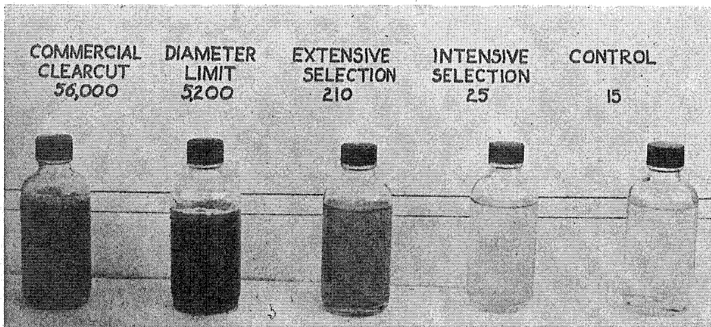
Figure 15.—Water samples showing maximum turbidities measured on each of the five gaged watersheds. Differences are due largely to differences in skidroad layout and construction.
