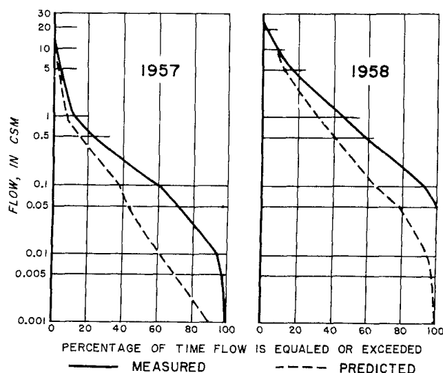
Figure 24.—Flow-duration curves for Clearcut Watershed for growing seasons in 1957 and 1958.
