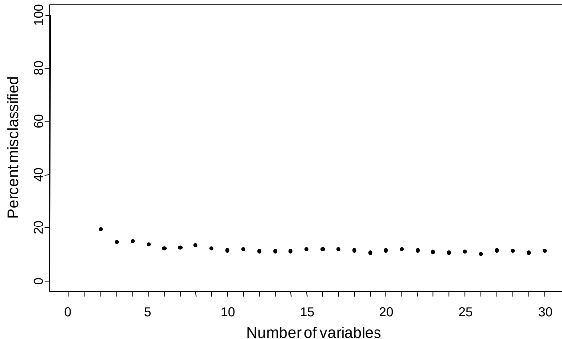
Figure 4. Out-of-bag error estimate of classification and regression trees as a function of the number of variables included from 300 iterations of random forest classification and regression tree analyses. Including more than 3 variables in the classification and regression tree does not substantially reduce the misclassification rate.
