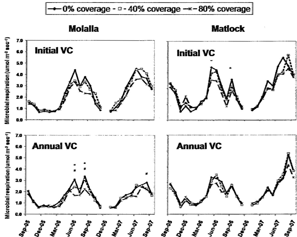
Fig. 4. Microbial soil respiration by sample month and logging-debris treatment with either initial or annual vegetation control (VC) at Molalla and Matlock. *Significant contrasts between the absence and presence of logging debris. #Between 40 and 80% logging-debris coverage. Only data from April to September in each year were analyzed.
