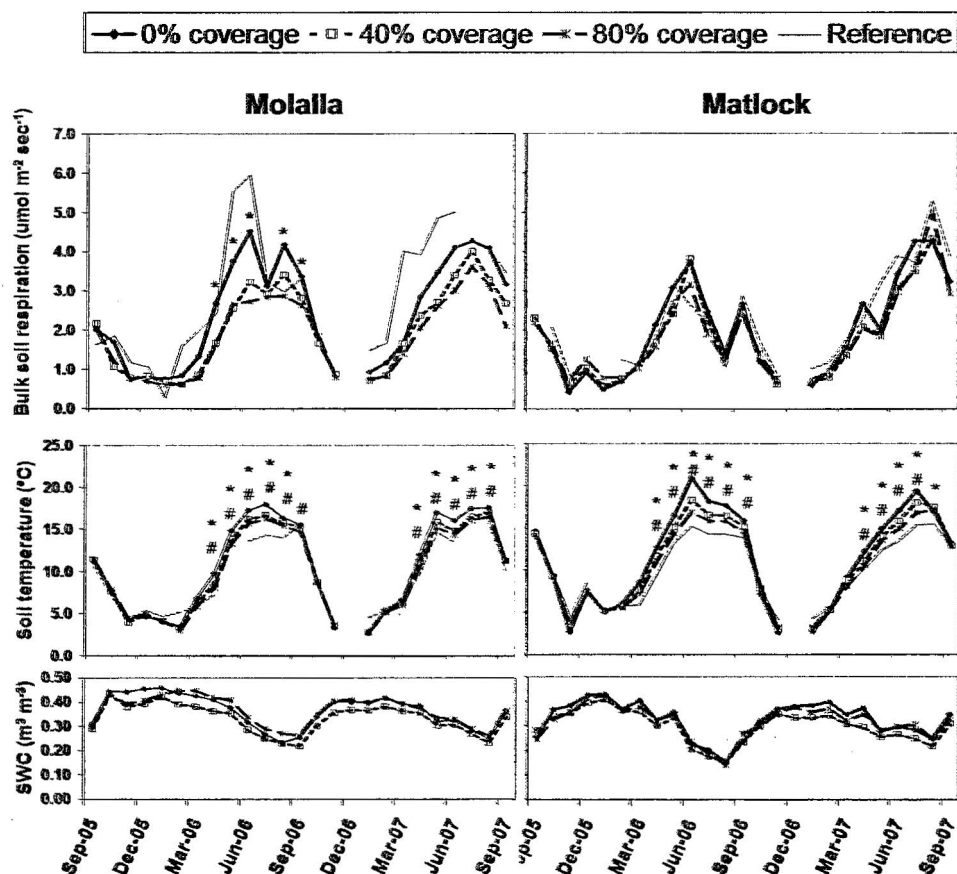
Fig. 3. Bulk soil respiration, soil temperature, and volumetric soil water content (SWC) by sample month and logging-debris treatment at Molalla and Matlock. *Significant contrasts between the absence and presence of logging debris. #Between 40 and 80% logging-debris coverage. Only data from April to September in each year were analyzed.
