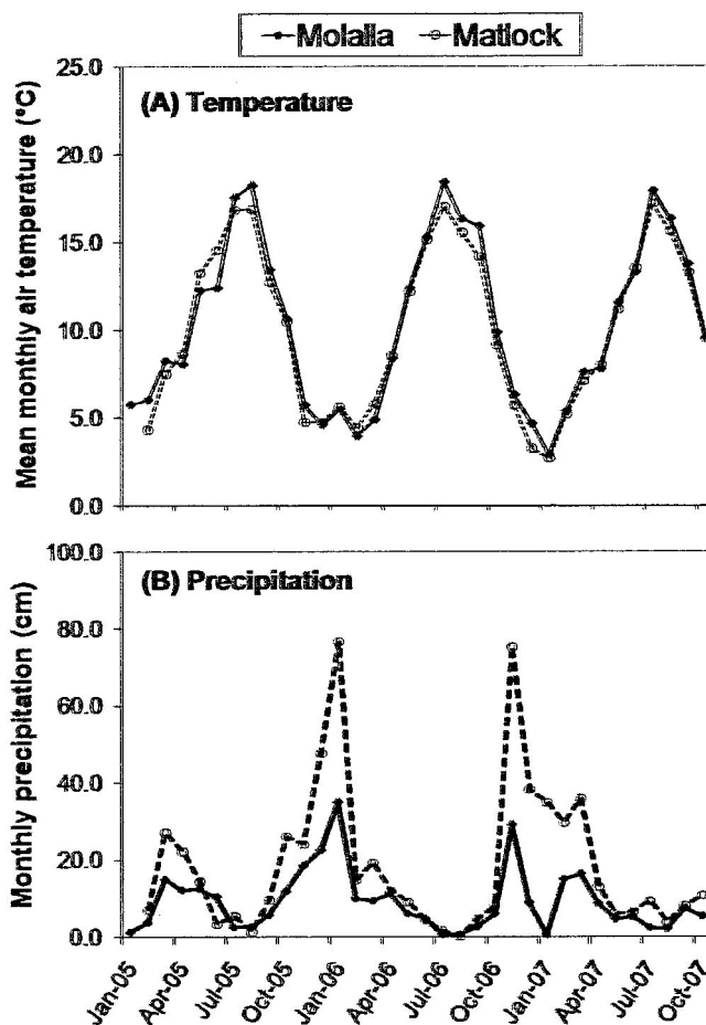
Fig. 1. Mean monthly (A) air temperature and (B) precipitation at Molalla and Matlock for the study duration.
