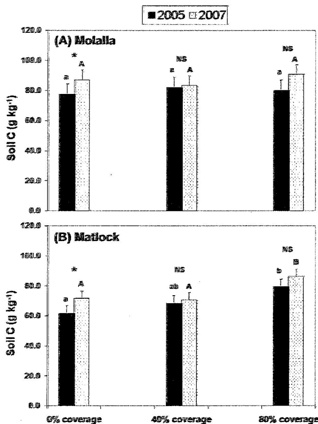
Fig. 5. Total soil C concentration to a depth of 20 cm by sample period and logging-debris treatment at (A) Molalla and (B) Matlock. Means within a year followed by a different letter (lowercase letters for 2005 and uppercase letters for 2007) are significantly different ( P \leq 0.05 ). *Significant ( P \leq 0.05 ) differences between the two measurement periods; NS, no significant difference between periods. Error bars are standard error of the mean.
