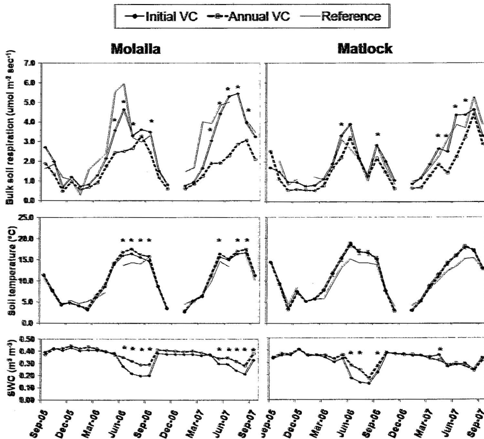
Fig. 2. Bulk soil respiration, soil temperature, and volumetric soil water content (SWC) by sample month and competing vegetation control (VC) treatment at Molalla and Matlock. *Significant difference between treatments for the associated month. Only data from April to September in each year were analyzed.
