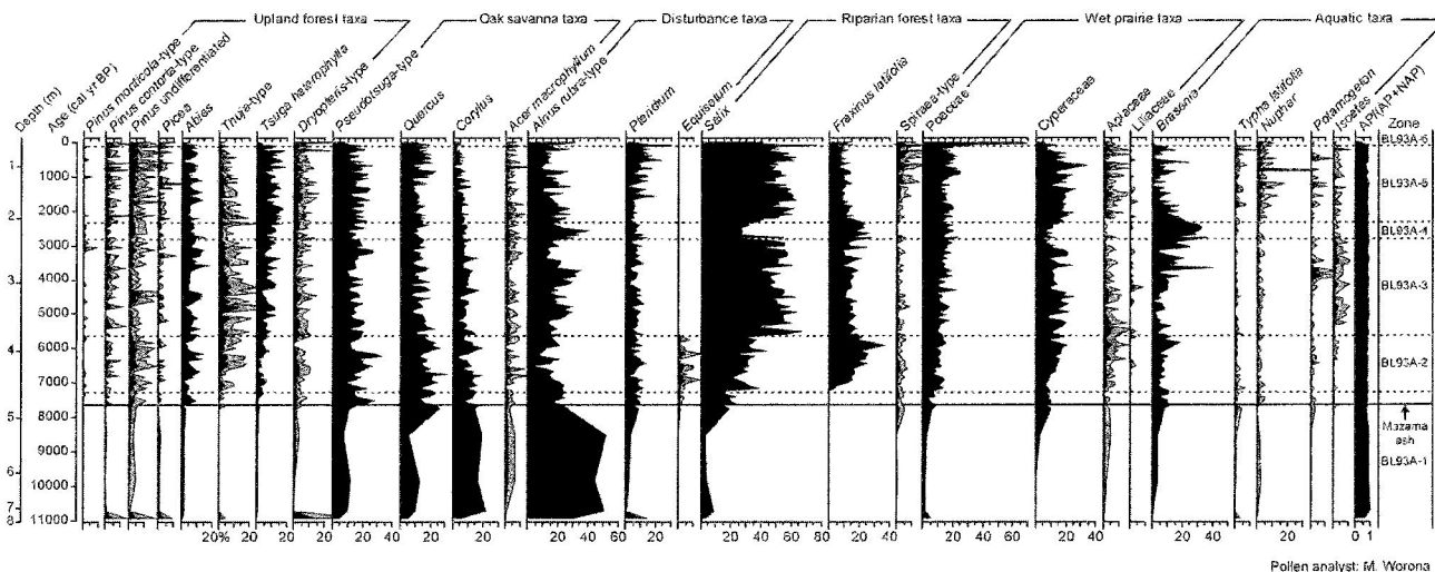
Fig. 5. Percentages of selected pollen taxa and spores, and AP/NAP ratio from core BL93A plotted against age (cal yr BP). Gray curves represent a 3X exaggeration of solid black curve. Dashed lines indicate zone boundaries.
