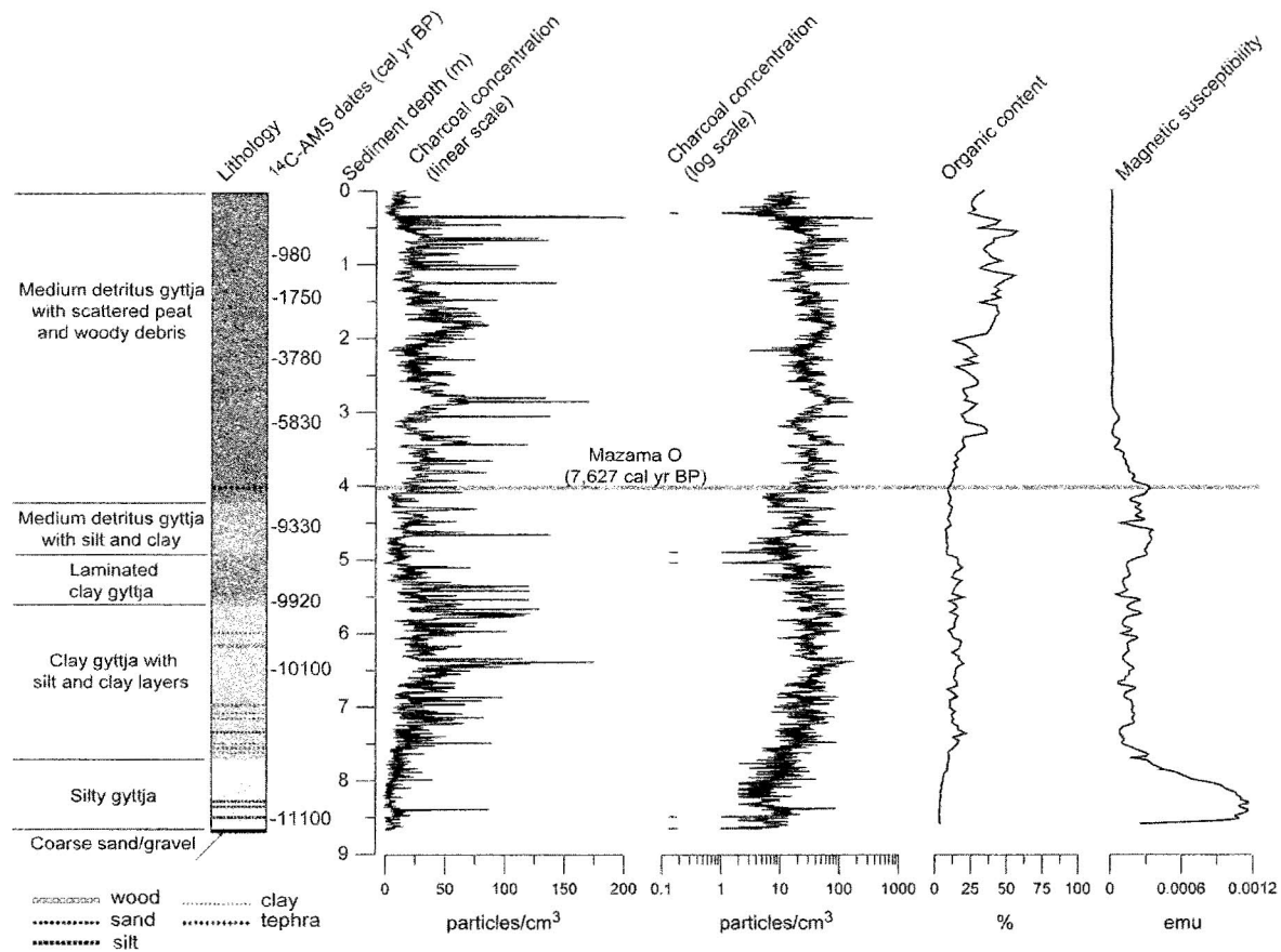
Fig. 4. Lithology, ^{14}\text{C} -AMS dates, charcoal concentration (linear scale), charcoal concentration (log scale), organic content, and magnetic susceptibility for core BL05B plotted against depth (m). The vertical ticks on the charcoal concentration (log scale) curve represent zero values.
