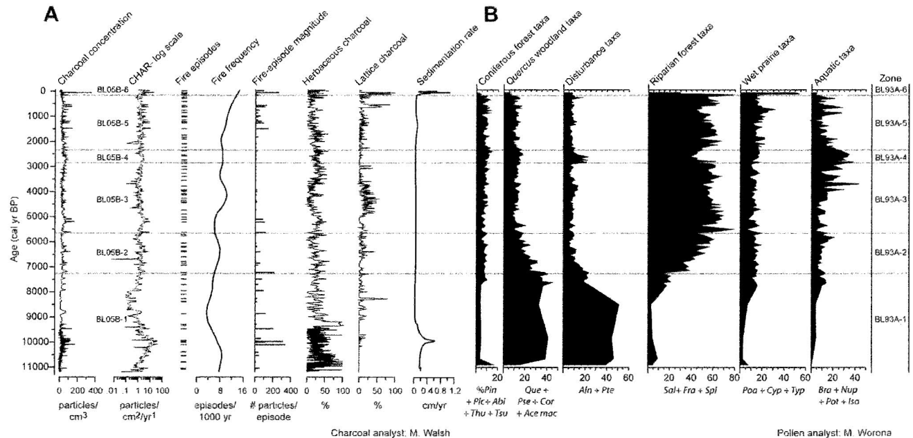
Fig. 7. A) Core BL05B charcoal concentration, charcoal accumulation rate (log scale), fire episodes, fire frequency, fire magnitude, herbaceous charcoal, lattice charcoal, and sedimentation rate plotted against age (cal yr BP). B) Core BL93A selected summed pollen percentages plotted against age (cal yr BP). Pollen abbreviations are as follows: Pic = Picea , Abi = Abies , Thu = Thuja plicata , Tsu = Tsuga heterophylla , Que = Quercus , Pse = Pseudotsuga menziesii , Cor = Corylus , Ace mac = Acer macrophyllum , Aln = Alnus rubra , Pte = Pteridium , Sal = Salix , Fra = Fraxinus latifolia , Spi = Spiraea , Poa = Poaceae , Cyp = Cyperaceae , Typ = Typha latifolia , Bra = Brasenia , Nup = Nuphar , Pot = Potamogeton , Iso = Isoetes .
