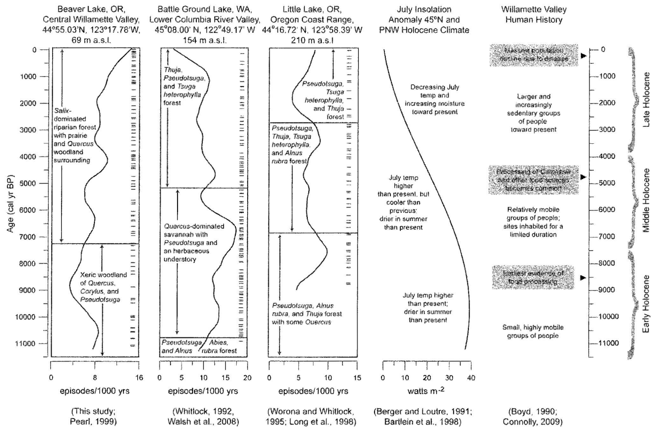
Fig. 8. Reconstructed vegetation, fire frequency, and fire episodes (peaks) plotted against age (cal yr BP) for Pacific Northwest sites. Sites are arranged from low to high elevation (left to right). Also shown are July insolation anomaly for 45°N latitude and Pacific Northwest Holocene climate history; and a generalized human history for the Willamette Valley, Oregon.
