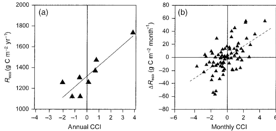
Fig. 7 Annual (a), ( R^2 = 0.75 , P < 0.01 ) and monthly (b), ( R^2 = 0.33 , P < 0.001 ) R_{eco} anomalies are positively related to the CCI. Reduced ecosystem respiration was observed during negative climate phases.
