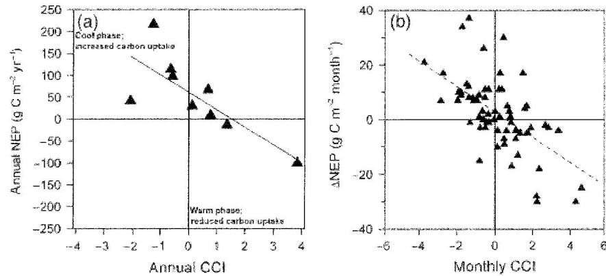
Fig. 5 Greater net carbon uptake is associated with more negative annual CCI ( R^2 = 0.55 , P < 0.01 ) (a). Monthly anomalies in NEP show more scatter ( R^2 = 0.34 ) but are significantly correlated ( P < 0.001 ) to the CCI (b).
