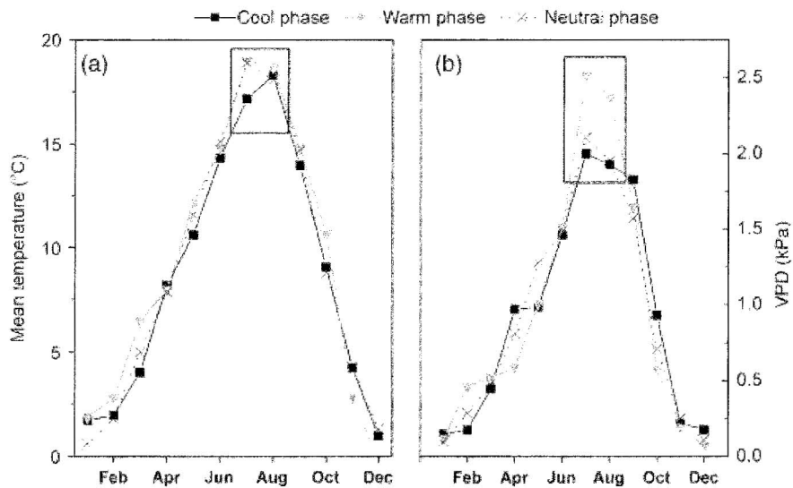
Fig. 4 Monthly average air temperature (a) and VPD (b) associated with positive (warm), negative (cool), and neutral climate phases from 1999 to 2007.
