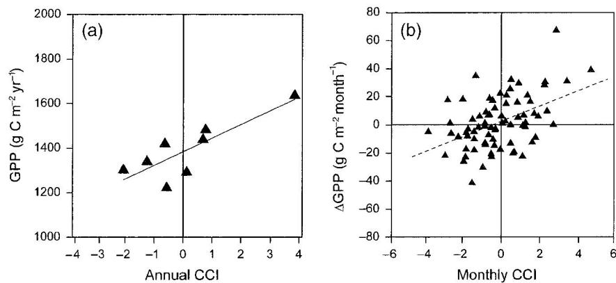
Fig. 6 Annual (a), ( R^2 = 0.64 , P > 0.01 ) and monthly (b), ( R^2 = 0.22 , P < 0.001 ) GPP anomalies are positively related to the CCI. Higher photosynthesis was observed during positive climate phases.
