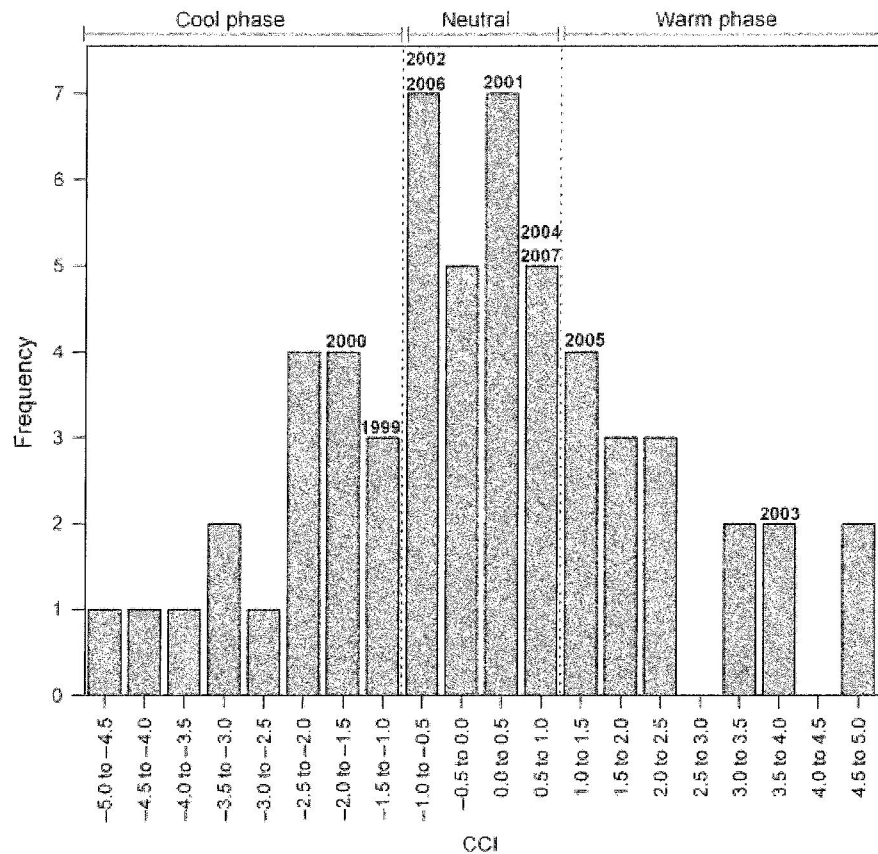
Fig. 2 The frequency of annual CCI magnitudes from 1950 to 2007 with the flux measurement years labeled.
