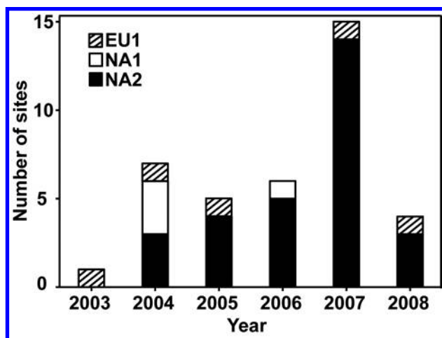
Fig. 1. Clonal lineage of Phytophthora ramorum isolates sampled from nurseries in British Columbia, Canada by year. Both an EU1 isolate and NA2 isolates were collected from a single site in 2007 and five sites are represented in multiple years, two of which had different lineages in different years.
