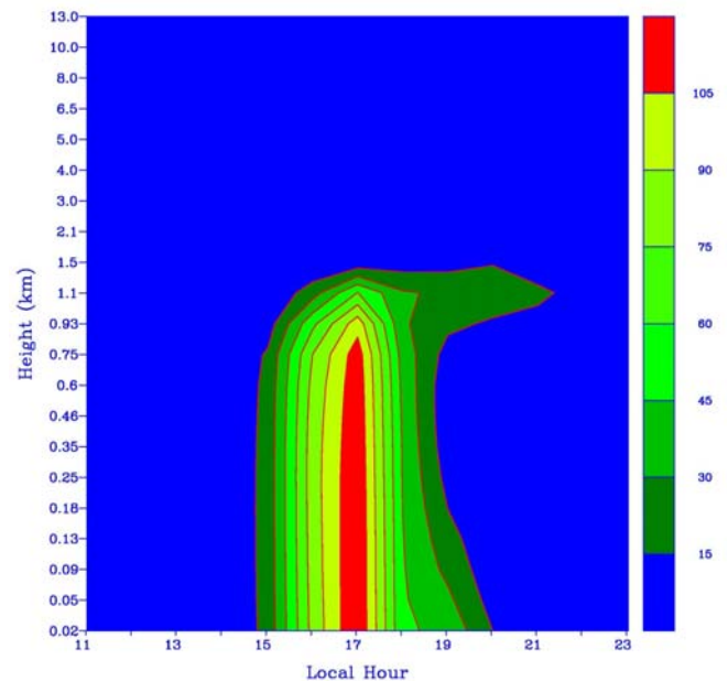
Figure 10. Same as Figure 9 except for 10 updraft cores.
