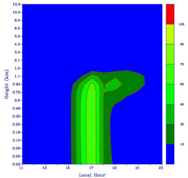
Figure 9. Time–height across section of PM_{2.5} concentration ( \mu g m^{-3} ) at Asheville simulated with CMAQ with Daysmoke simulation of plume rise for 1 updraft core.
