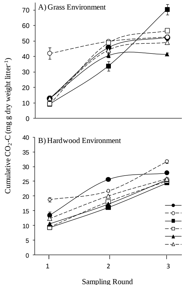
Fig. 1. Cumulative litter decomposition across each 100-day sampling round for six different microbial community inocula in grass (A) and hardwood (B) environments. Closed symbols and solid lines represent inocula from grassland sites and open symbols and dashed lines from hardwood sites. Values are means \pm 1 SE ( n = 6 ). For clarity, pair-wise comparisons are not shown. However, in each round at least three inocula are significantly different ( P \leq 0.05 ).
