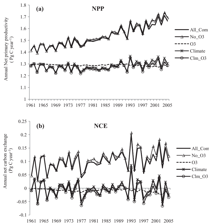
Figure 3 (a) Changes of annual net primary productivity (NPP; Pg C year -1 ) and (b) annual net carbon exchange (NCE; Pg C year -1 ) between forest ecosystems and atmosphere during 1961–2005 under different simulation experiments. Note: the All_Com scenario considers all the environmental factors including O 3 pollution, climate, nitrogen deposition, CO 2 , land-cover and land-use change; No_O 3 means the All_Com without O 3 effects; O 3 , Climate and Clm_O 3 are simulation experiments of O 3 only, climate only and a combination of climate and O 3 .
