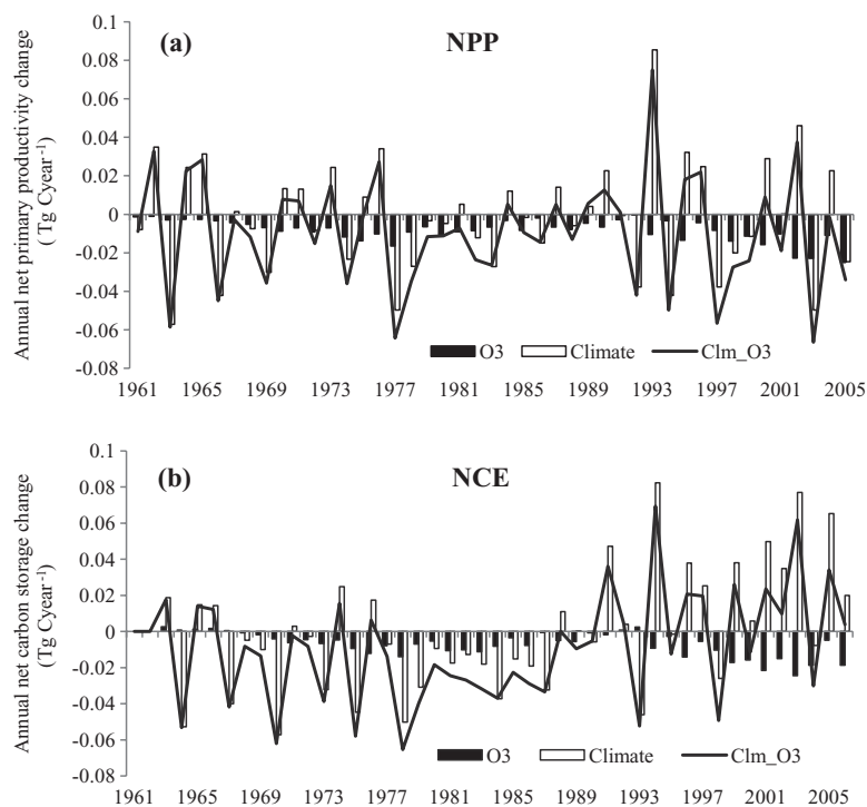
Figure 6 Annual changes in relative contributions of ozone pollution, climate change and their interaction to (a) annual net primary productivity (NPP) and (b) net carbon storage ( \text{Tg C year}^{-1} ). Note: O 3 , Climate and Clm_O 3 are simulation experiments of O 3 only, climate only and a combination of climate and O 3 .
