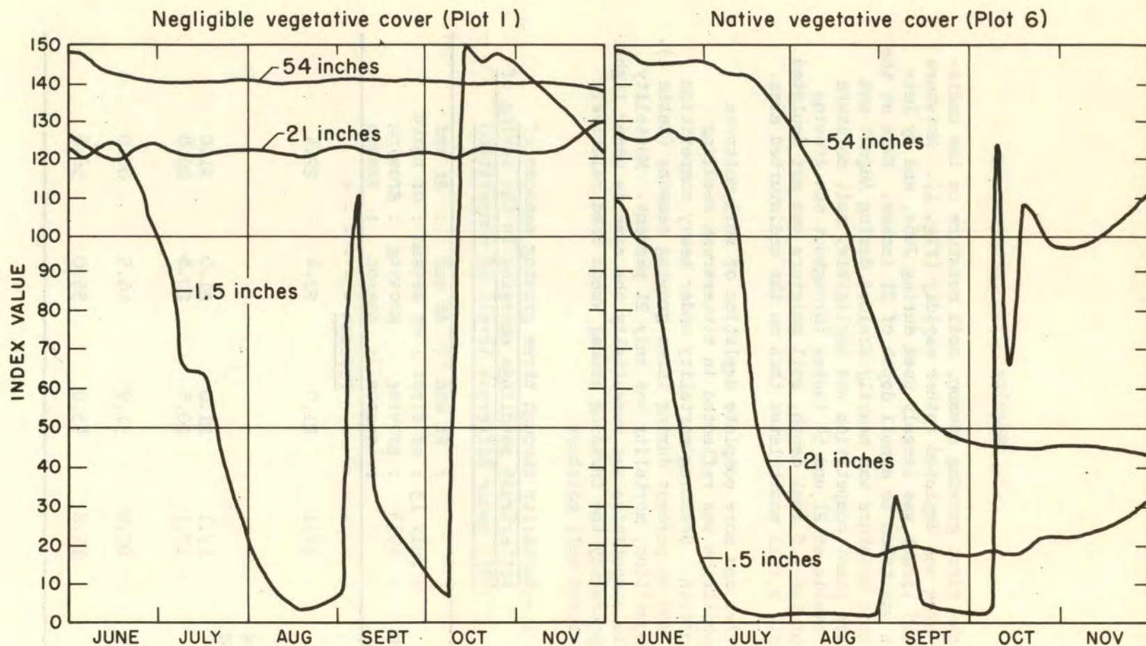
Figure 1.--Trends of soil moisture indices at three soil depths--1.5, 21, and 54 inches--under negligible and native vegetative cover during the first growing season (1953). Indices of 120 to 150 are in the range of high soil moisture; 0 to 30, in the range of low soil moisture.
