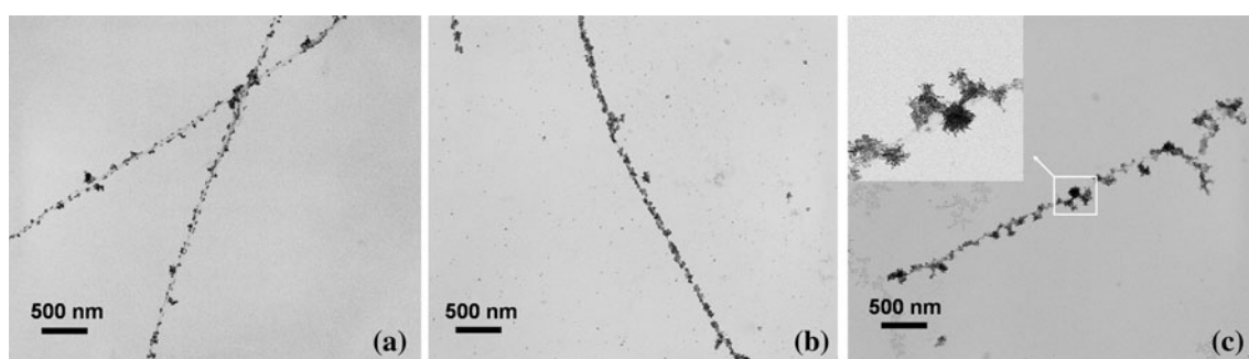
Fig. 7 TEM images of CdS samples with varying \text{H}_2\text{S} exposure time of 2 min (a), 5 min (b), and 10 min (c)
