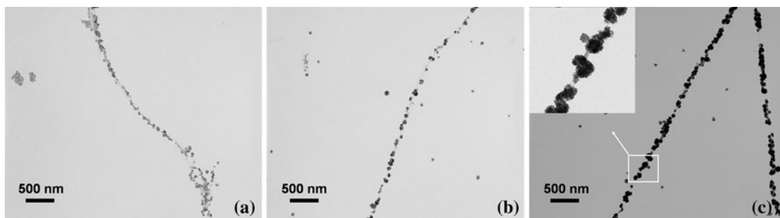
Fig. 9 TEM images of ZnS samples with varying \text{H}_2\text{S} exposure time of 2 min (a), 5 min (b), and 10 min (c)
