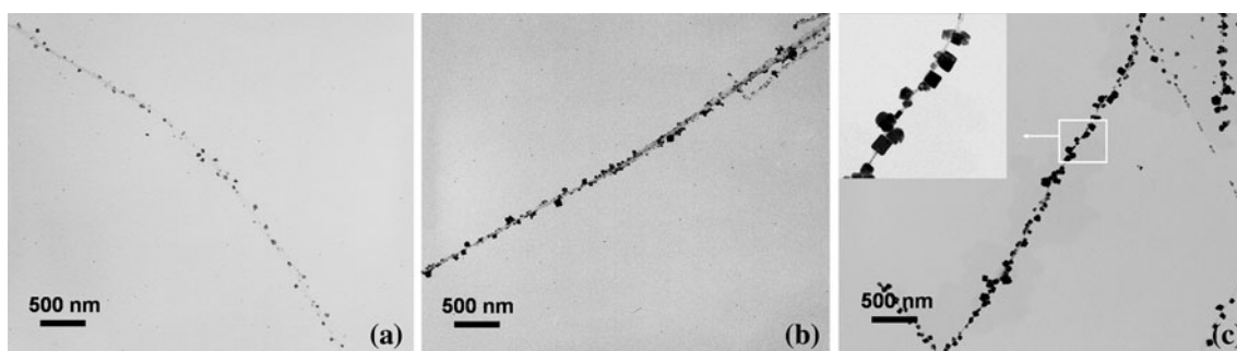
Fig. 8 TEM images of PbS samples with varying \text{H}_2\text{S} exposure time of 2 min (a), 5 min (b), and 10 min (c)
