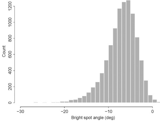
Figure 4. Histogram of the broadened left half-profile bright spot associated with the left face of a rectangular wood cell when cell rotation = 0°, cell tilt = 0°, and microfibril angle = 30°. The skewness of this distribution was -1.28. This figure was generated by calculating left half-profile, left face bright spot locations associated with 10,000 microfibril angle draws from a Gaussian distribution centered at 30° with variance (30/3)^2 + 6 .
