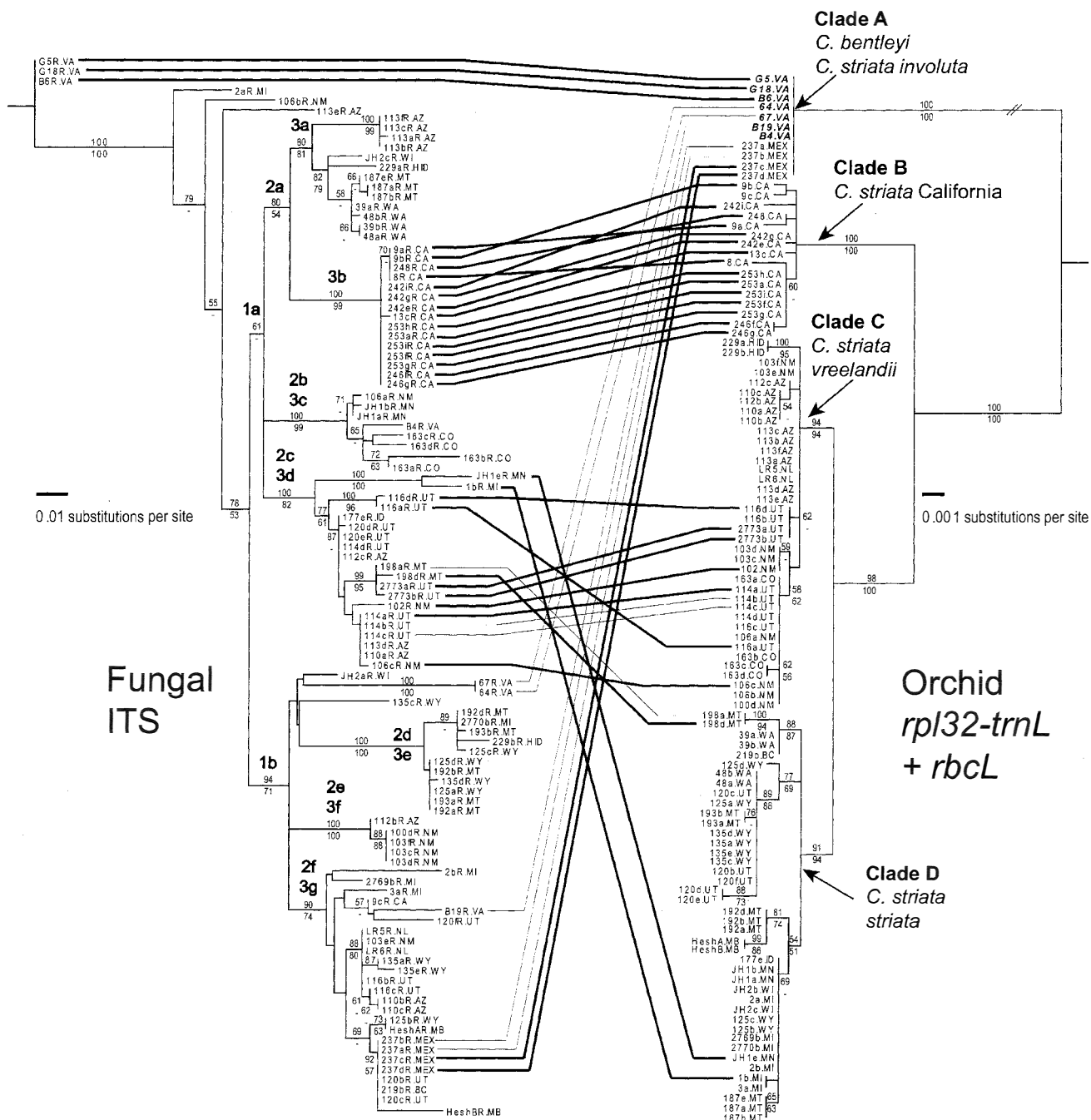
Fig. 3. Cophylogenetic analysis of fungal ITS (left; using the striata -only matrix) and orchid rbcL + trnL (right) gene trees. Trees are represented by highest likelihood topologies under the GTRGAMMA model in RaxML. Two values are displayed for each branch: numbers above are ML bootstrap values based on 2000 replicates (above), and numbers below are results of 10 000 maximum parsimony (MP) jackknife replicates from TNT (support values <50 are indicated by a “-” symbol). Larger numbers in boldface above support values in the fungal ITS gene tree are clade assignments for contingency tests, representing multiple levels (1a–b; 2a–f; 3a–g; see Appendix 3). Bold lines connecting accessions between the trees indicate significance for both MP and maximum likelihood (ML) input trees of that particular association at the P = 0.05 significance level based on 9999 ParaFit permutations. Thin lines indicate significance in either MP or ML (see Appendix 3). Left scale bar (fungi) = 0.01 substitutions per site and right scale bar (orchids) = 0.001 substitutions per site. “R” in each C. striata accession name indicates that the fungal ITS sequence was obtained from rhizome DNA.
