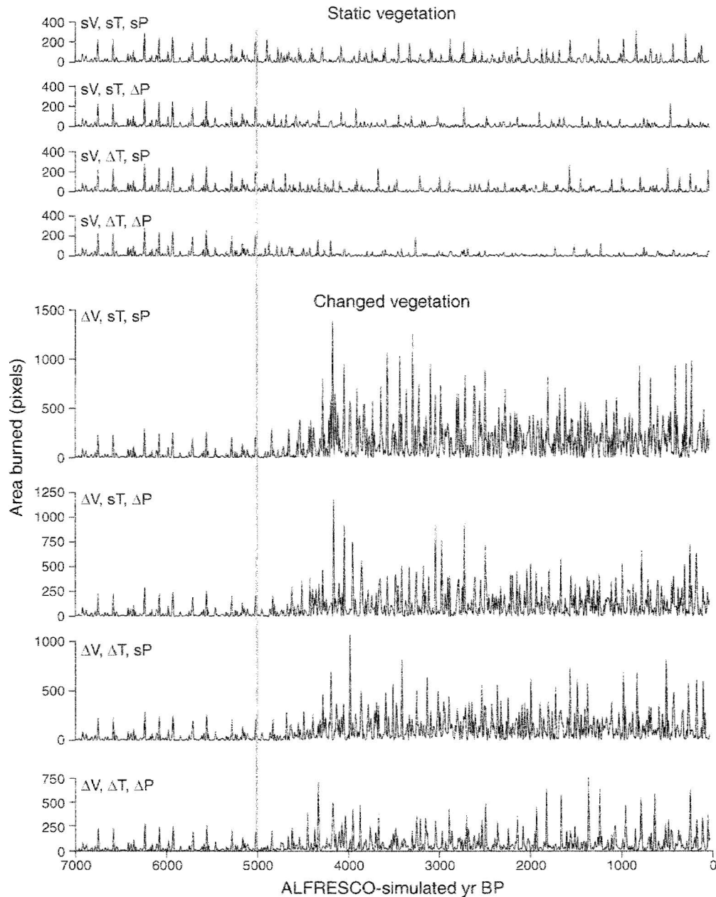
FIG. 5. Time series of area burned for ALFRESCO simulations. The gray line separates the two simulation periods.
