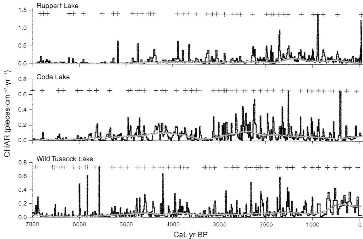
FIG. 4. CHAR records for Ruppert, Code, and Wild Tussock lakes over time (calibrated years before present). Plus signs (+) indicate inferred fire events at each site.
