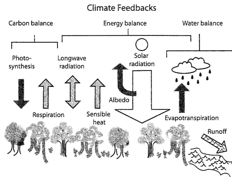
Fig. 3. Three major categories of climate feedbacks (each shown by the arrows beneath the bracket) between ecosystems and the climate system. Each of these ecosystem–atmosphere exchanges influences climate. Cooling effects on climate are shown by black arrows; warming effects by grey arrows. Arrows show the direction of the transfer; the magnitude of each transfer differs among ecosystems. The effects of aerosols and surface roughness are not shown. Redrawn from Chapin et al. (2008).
