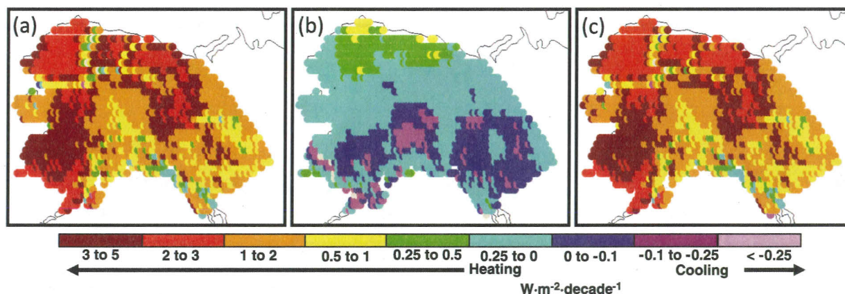
Fig. 3. Changes in energy ( \text{W}\cdot\text{m}^{-2}\cdot\text{decade}^{-1} ) due to changes in (a) the timing of snowmelt, (b) the timing of snow return, and (c) the length of the snow cover duration in the western Arctic between 1970 and 2000. Further details are in Euskirchen et al. 2007.
