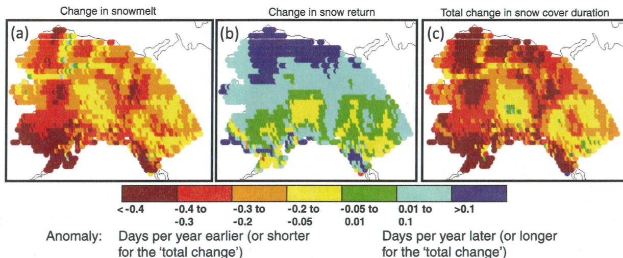
Fig. 2. Spatial distribution of changes in snow cover (days-year -1 ) for changes in (a) snowmelt, (b) snow return, and (c) the total length of the snow cover duration in the western Arctic between 1970 and 2000. Further details are in Euskirchen et al. 2007.
