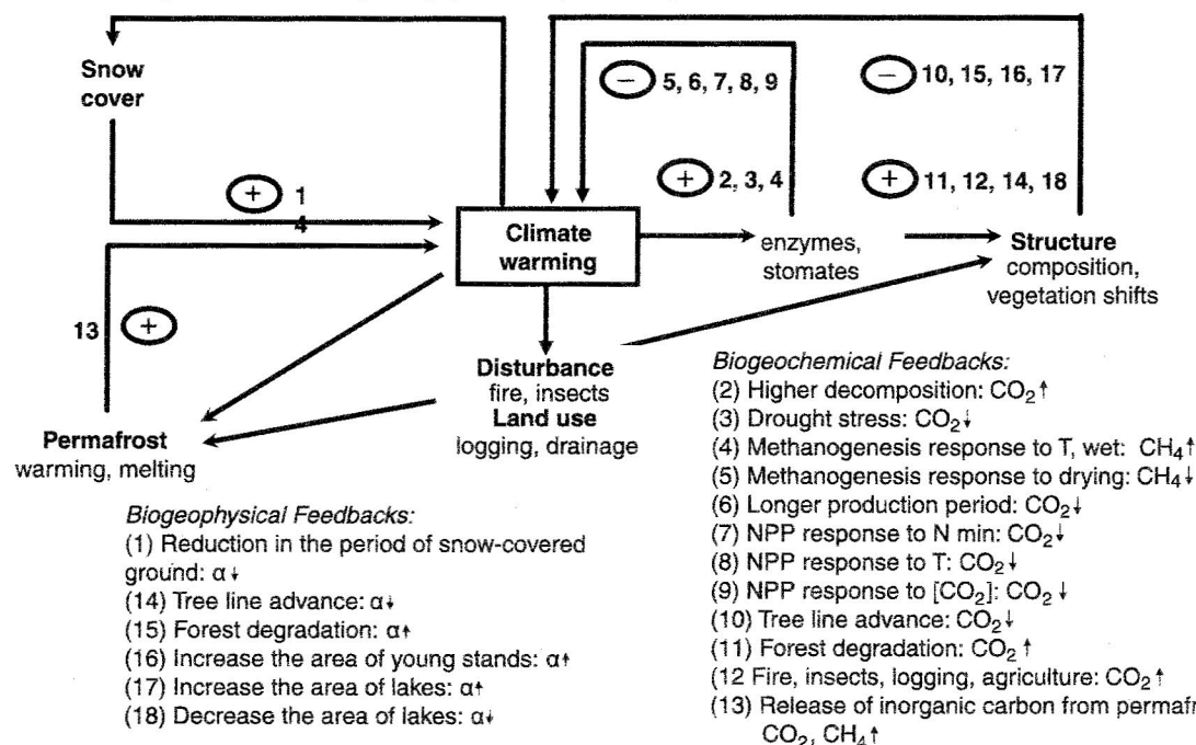
Fig. 1. Conceptualization of the climate feedbacks in Alaska's boreal forests. \alpha , albedo; +, positive feedback to climate; -, negative feedback to climate. T, temperature; NPP, net primary productivity; N, nitrogen. Modified after McGuire et al. 2006.
