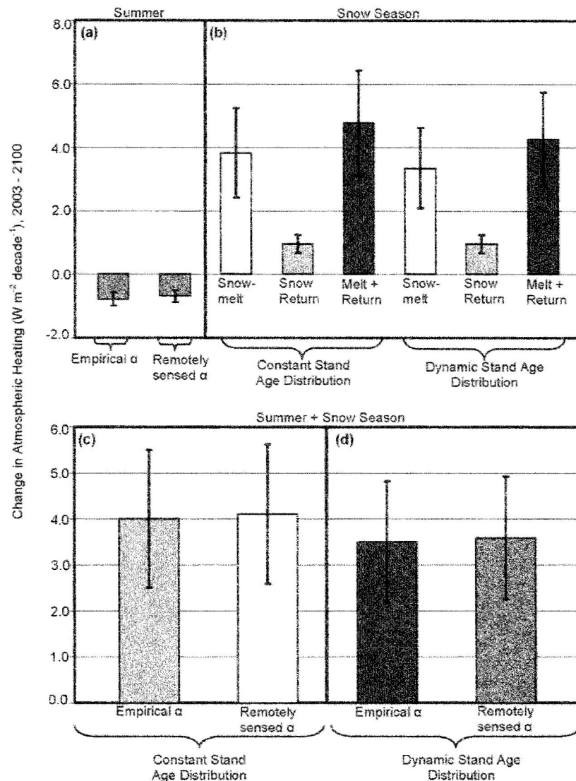
Figure 6. Mean changes in atmospheric heating from 2003 to 2100 across all four input climate scenarios ( \text{W m}^2 \text{ decade}^{-1} , \pm standard deviation). (a) The changes in atmospheric heating are due to summer albedo change based on both empirical and remotely sensed estimates of albedo ( \alpha ). (b) The changes in atmospheric heating are due to the snow season albedo changes, taking into account both a constant forest stand age distribution and a dynamic forest stand age distribution. (c) The changes in atmospheric heating for the summer and snow season are summed and are based on the constant forest stand age distribution for the snow season. (d) The changes in atmospheric heating for the summer and snow season are summed and incorporate the dynamic stand age distributions for the snow season.
