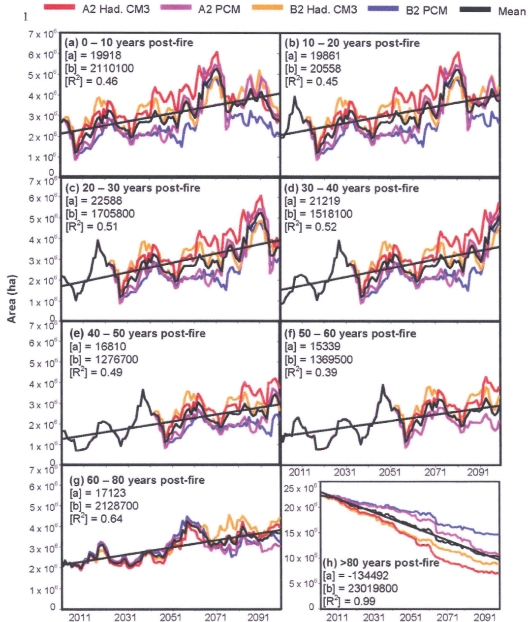
Figure 4. Changes in the distribution of the age of the ecosystems postfire based on ALFRESCO simulations. A least squares regression line is fit to the means of the data, with p < 0.0001 for all regressions in Figures 4a–4c. [a] is slope, and [b] is intercept.
