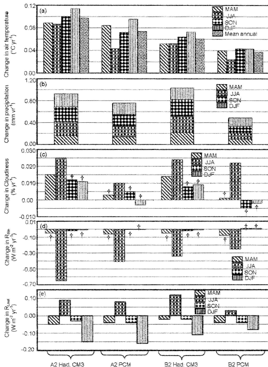
Figure 2. Trends in (a) air temperature, (b) precipitation, (c) cloudiness, (d) incoming shortwave solar radiation ( R_{\text{Sin}} ), and (e) net longwave radiation ( R_{\text{Lnet}} ) in the western Arctic between 2003 and 2100 based on two climate models and scenarios. Trends are based on the slopes of least squares linear regression. All trends in air temperature, precipitation, and R_{\text{Lnet}} were statistically significant at p < 0.0001 . For cloudiness and R_{\text{Sin}} , trends marked with daggers were not statistically significant at p < 0.0001 . MAM, March, April, and May; JJA, June, July, and August; SON, September, October, and November; DJF, December, January, and February; Mean is the mean across all scenarios and climate models.
