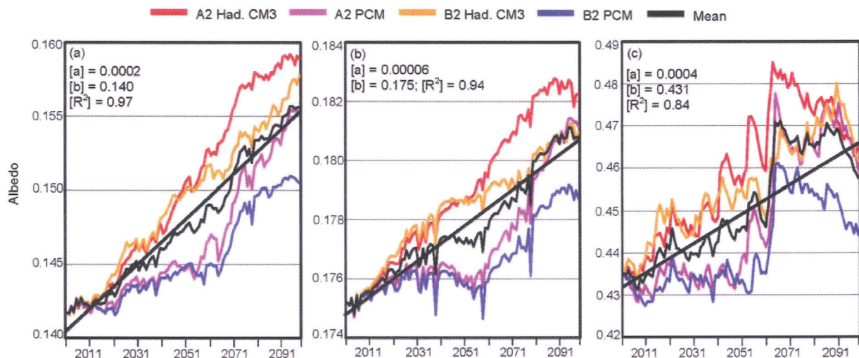
Figure 5. Changes in albedo due to the changes in the postfire distributions of the ecosystems over the study region for the years 2003–2100. (a) These changes are based on Amiro et al. [2006] equations for summer albedo. (b) These changes are based on Randerson et al. [2006] and Lyons et al. [2008] equations for summer albedo. (c) These changes are based on Amiro et al. [2006] equations for snow season albedo. A least squares regression line is fit to the means of the data, with p < 0.0001 for all regressions in Figures 5a–5c. [a] is slope, and [b] is intercept.
