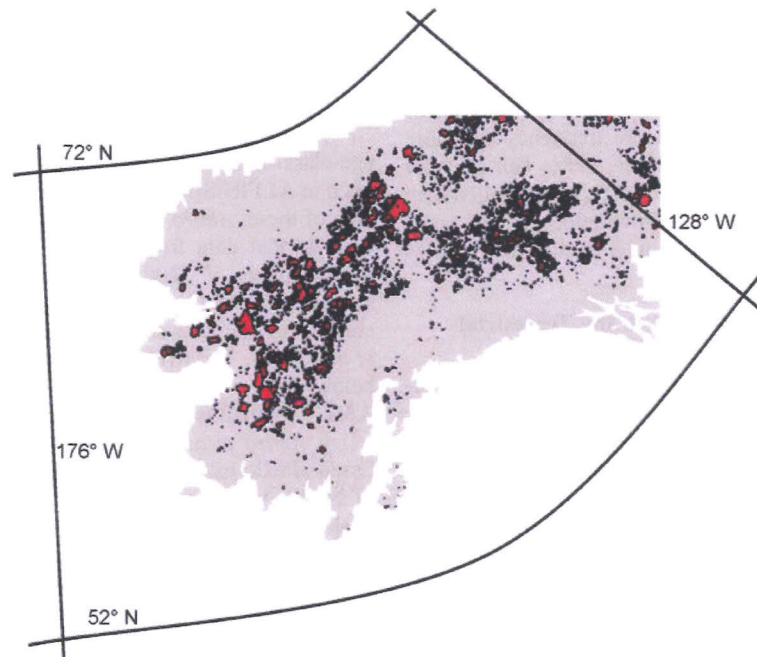
Figure 1. Map of the study domain, the western Arctic, and the perimeters of large fires between 1950 and 2000.
