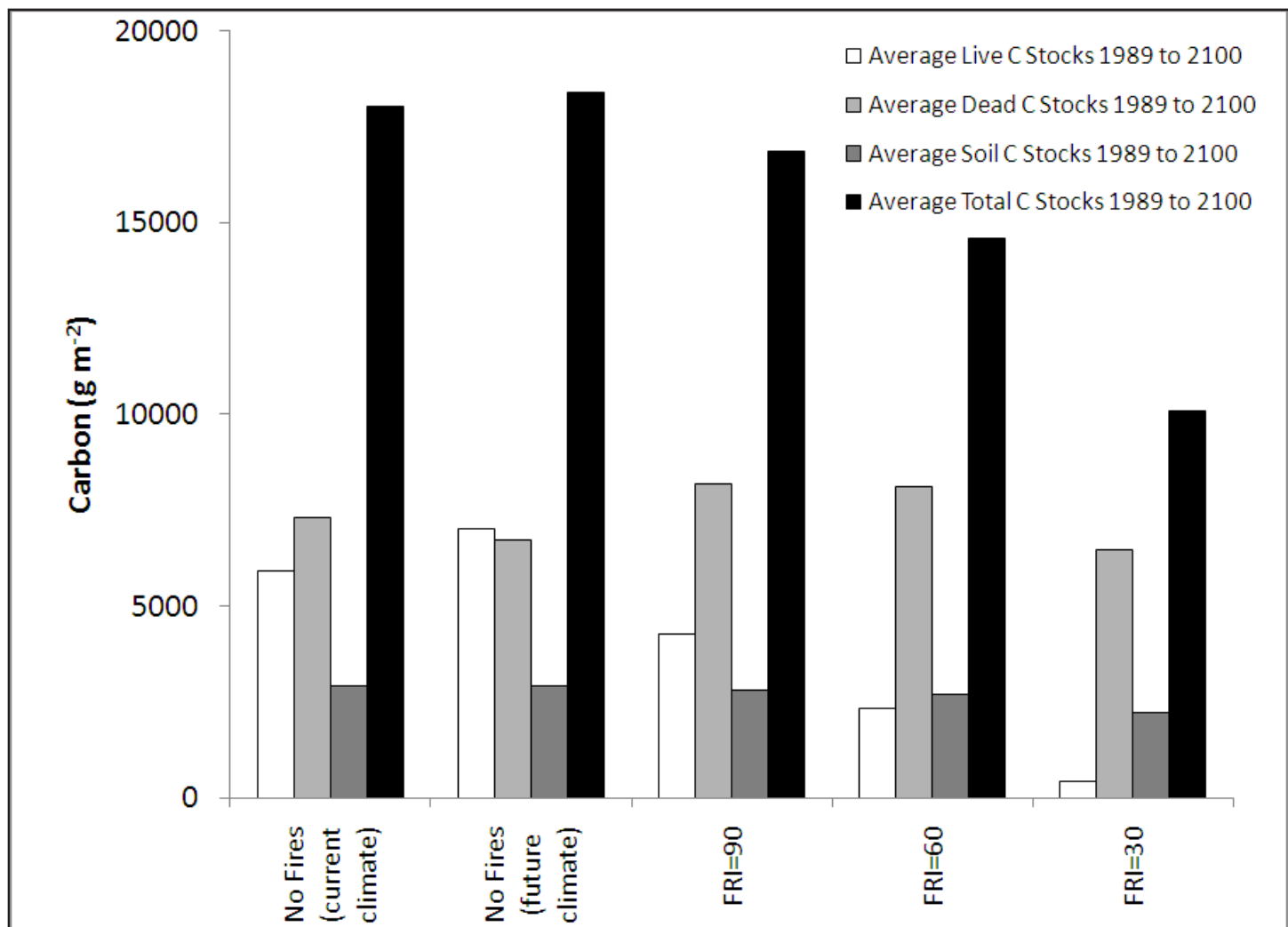
Figure 2. Carbon stocks ( \text{g m}^{-2} ) for live, dead, soil, and total forest pools for historical (no fires between 1989 and 2100) and future fire (90-, 60-, or 30-year fire return interval (FRI)) under current or future climate. Future climate was averaged across three climate scenarios (see text).
