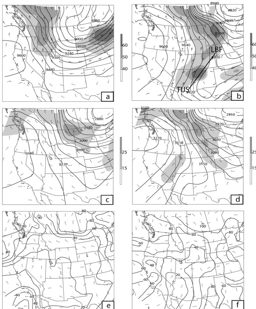
FIG. 5. Barnes analysis of (a), (b) 300- and (c), (d) 700-hPa geopotential height (solid lines; m), wind speed (shaded) and wind barbs, and (e), (f) surface RH (solid lines; %) and wind barbs valid at (left) 0000 UTC 25 Oct and (right) 1200 UTC 26 Oct 2003. A long (short) wind barb denotes 10 (5) \text{m s}^{-1} . A flag denotes 50 \text{m s}^{-1} . Boldface solid line in (b) denotes cross-section location in Fig. 9.
