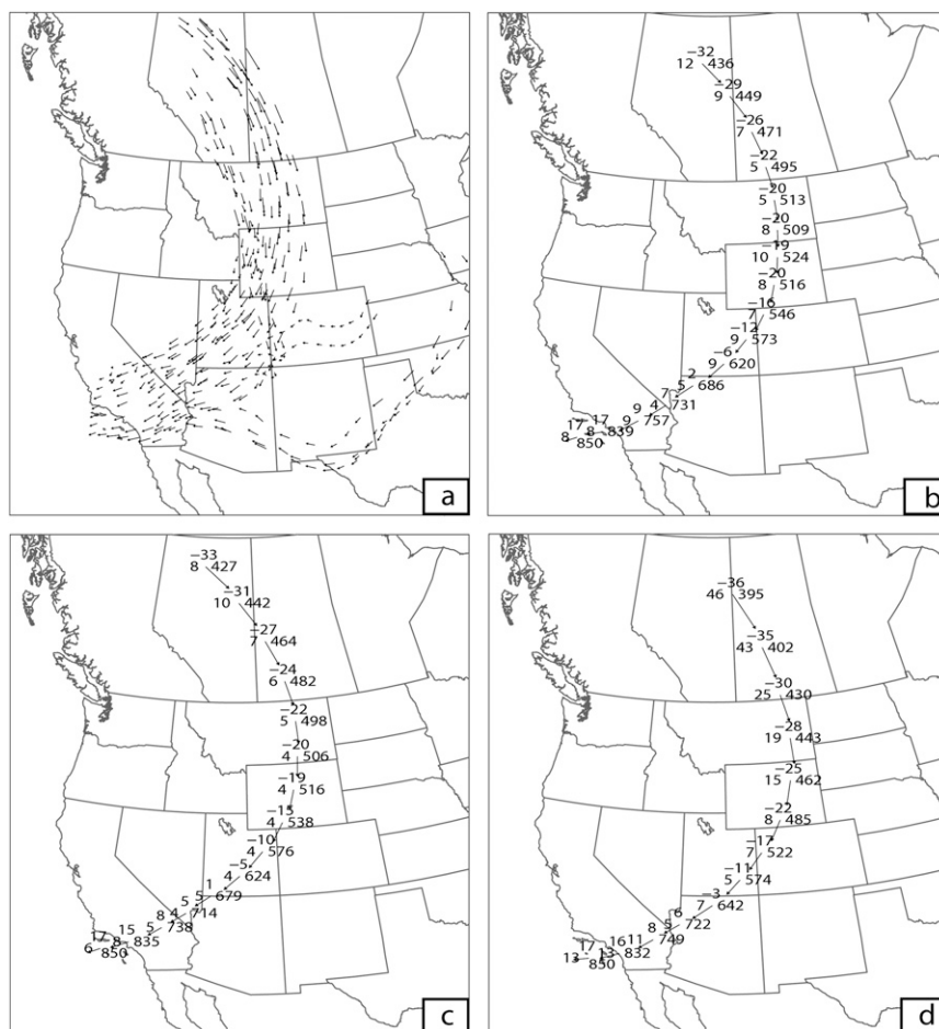
FIG. 14. Backward trajectories of (a) the winds for all 24 parcels, and the winds for parcels (b) A, (c) B, and (d) C from the 32-km NHMASS simulation starting at 0000 UTC 27 Oct 2003 back to their original positions at about 0300 UTC 25 Oct 2003. Trajectories are 3-hourly and caption is denoted below the figure: T is temperature ( ^{\circ}\text{C} ), RH is relative humidity (%), and P is pressure (hPa). Vectors denote winds with length proportional to wind speed.
