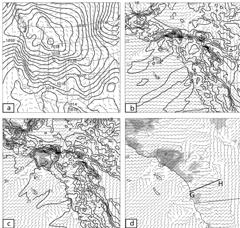
FIG. 20. (a) Sea level pressure (solid; hPa) and wind barbs at 1200 UTC 25 Oct 2003 from the 32-km simulation. (b) Surface mixing ratios (shaded for dry areas with values smaller than 2 \text{ g kg}^{-1} ), temperature (solid; ^{\circ}\text{C} ), and wind barbs valid at 1200 UTC 26 Oct 2003 from the 2-km simulation. (c) As in (b) but at 2100 UTC 26 Oct 2003. (d) Surface RH (shaded for dry areas with \text{RH} < 15\% ) and wind barbs valid at 2100 UTC 26 Oct from the 2-km simulation. Wind barb symbols are the same as in Fig. 5. The boldface solid line in (d) denotes the location of the cross section in Fig. 21.
