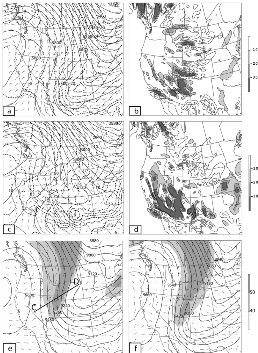
FIG. 13. (left) The 32-km NHMASS simulated geopotential height (solid; m), temperature (dashed; ^{\circ}\text{C} ), and wind barbs and (right) the temperature advection by the total wind at (a),(b) 500 and (c),(d) 700 hPa valid at 1200 UTC 26 Oct 2003. Ageostrophic wind barbs, total wind speed (shaded; \text{m s}^{-1} ), and geopotential height (solid; m) at 300 hPa valid at (e) 1800 UTC 25 Oct and (f) 0600 UTC 26 Oct 2003. Warm advection is denoted by solid contours and cold advection is shaded for values smaller than -10 \times 10^{-5} \text{ K s}^{-1} . Wind barb symbols are the same as in Fig. 5. Boldface line in (e) denotes cross-section location for Fig. 19b.
