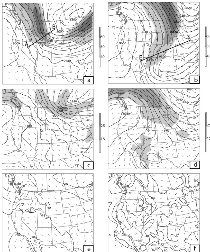
FIG. 10. Analysis of (a),(b) 300- and (c),(d) 700-hPa isotachs (shaded; \text{m s}^{-1} ), geopotential height (solid; m), and wind barbs ( \text{m s}^{-1} ), and (e),(f) surface RH (solid; %) and wind barbs ( \text{m s}^{-1} ) from the 32-km simulation valid at (left) 0000 UTC 25 Oct and (right) 1200 UTC 26 Oct 2003. Wind barb symbols are the same as in Fig. 5. Boldface lines in (a),(b) denote cross-section locations for Figs. 19a and 19c but are valid at 0300 UTC 25 Oct and 1200 UTC 26 Oct, respectively.
