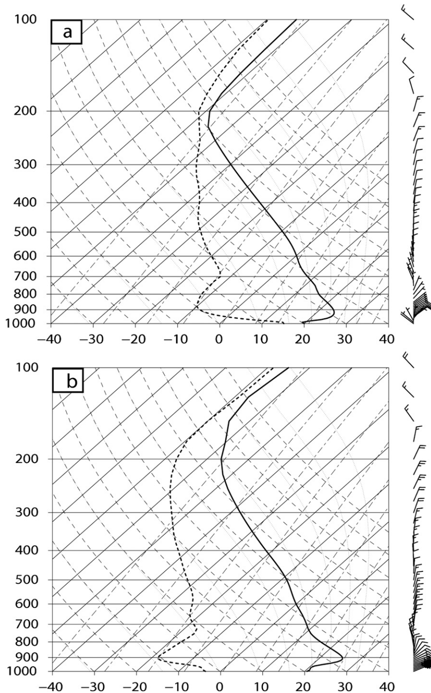
FIG. 22. Thermodynamic diagrams of temperature (solid) and dewpoint temperature (dashed) and the wind profile at KNKX valid at (a) 1800 UTC 25 Oct and (b) 1000 UTC 26 Oct 2003 from the 8-km NHMASS simulation.
