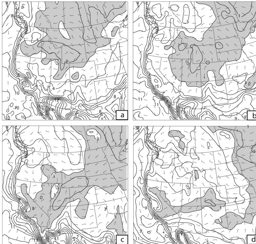
FIG. 15. Surface wind barbs and mixing ratios ( \text{g kg}^{-1} ; shaded for dry areas with values <3 \text{ g kg}^{-1} ) from the 32-km NHMASS simulation valid at (a) 1200 UTC 25 Oct, (b) 0000 UTC 26 Oct, (c) 1200 UTC 26 Oct, and (d) 0000 UTC 27 Oct 2003.
