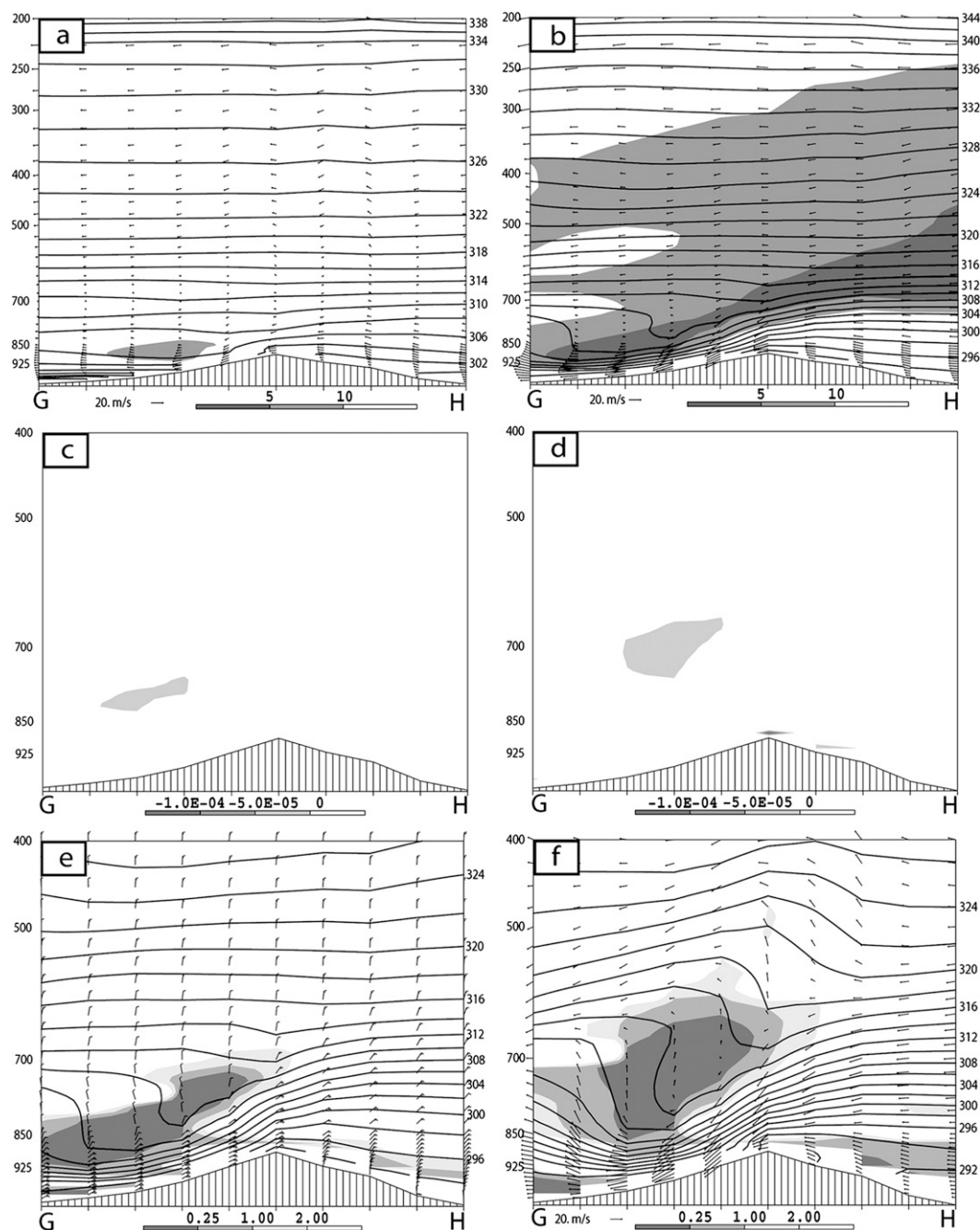
FIG. 21. Cross-section analyses along GH (denoted in Fig. 20d) from the 8-km simulation of RH (%), circulations (vectors), and \theta (solid; K) valid at (a) 1800 UTC 25 Oct and (b) 1000 UTC 26 Oct 2003. Here, N^2 (shaded for values < -5 \times 10^{-5} \text{ s}^{-2} ) are valid at (c) 1000 UTC 26 Oct and (d) 1800 UTC 26 Oct 2003. (e) The Ri (shaded for value < 2 ), \theta , and wind barbs valid at 1000 UTC 26 Oct and (f) the Ri, \theta , and circulations (vectors) valid at 1800 UTC 26 Oct 2003. Wind barb symbols are the same as in Fig. 5.
