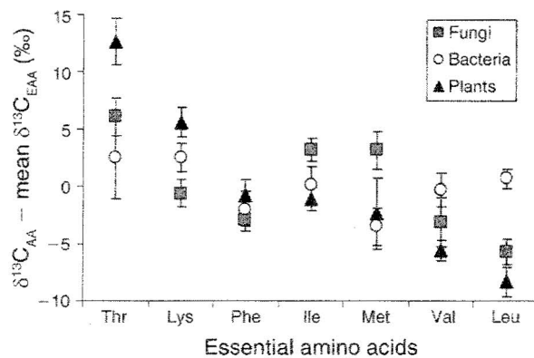
FIG. 1. The \delta^{13}\text{C} values of individual essential amino acids (EAA) for each taxon, relative to their respective mean EAA \delta^{13}\text{C} . The error bars show \pm SD of each taxon. The statistical significance of contrasts between the taxa is given in Table 2. Abbreviations are: Thr, threonine; Lys, lysine; Phe, phenylalanine; Ile, isoleucine; Met, methionine; Val, valine; Leu, leucine.
