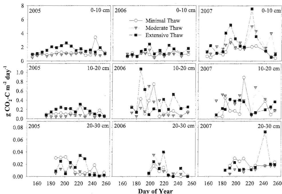
Figure 3. Soil profile CO 2 fluxes for the three sites during the growing season (June–August) from 2005 to 2007 calculated for 10 cm intervals. Each symbol of soil CO 2 fluxes represents a weekly mean averaged by site. Note the scale of the y axis changes for each different depth interval.
