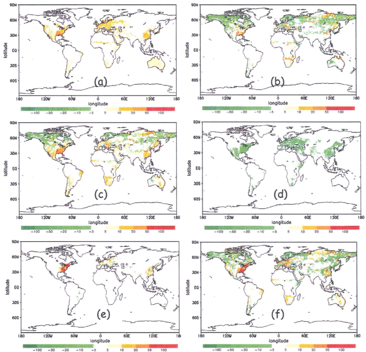
Figure 4. Spatial distributions are shown of the difference in modeled carbon flux to the atmosphere ( \text{gC m}^2 \text{yr}^{-1} ) between the with- and without-N dynamics cases (ISAM-NC minus ISAM-C) during the 1990s driven by changes in (a) concentrations of atmospheric \text{CO}_2 , (b) climate (temperature and precipitation), (c) \text{CO}_2 and climate, (d) nitrogen deposition, (e) LCLUCs, and (f) \text{CO}_2 , climate, nitrogen deposition, and LCLUCs. The modeled change in carbon storage, due to the addition of nitrogen dynamics, leads to additional carbon storage in the terrestrial biosphere where values are negative and reduced storage where values are positive.
