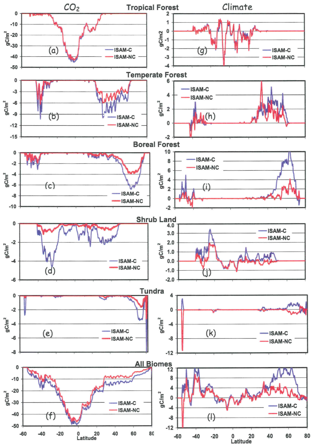
Figure 5. ISAM-estimated global and annual-mean latitudinal distribution of net carbon flux of carbon ( \text{gC m}^2 \text{ yr}^{-1} ) for the 1990s as a result of changes in concentrations of (left) atmospheric \text{CO}_2 and (right) climate (temperature and precipitation) for different individual biomes and all biomes. The results are compared for cases where C fluxes are constrained by N cycle (ISAM-NC) and C fluxes are not constrained by N cycle (ISAM-C).
