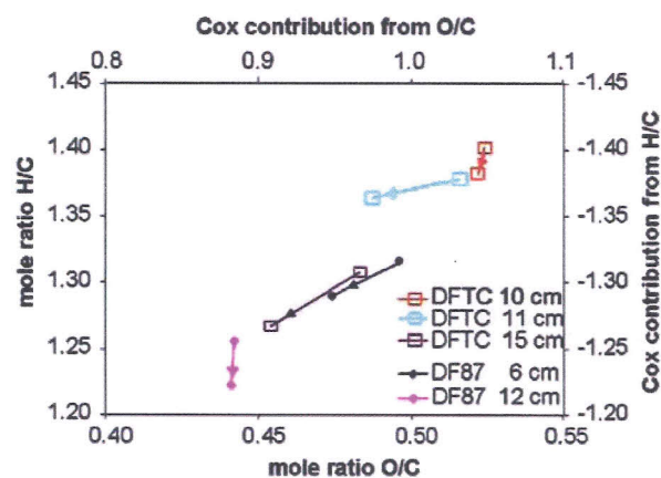
Figure 4. Vector diagram showing the trajectory of changes in C_{ox} and elemental composition caused by HF treatment. Values are calculated from CP NMR spectra by the molecular mixing model. Soil samples correspond to those in Table 2 from near Delta Junction Alaska. Open symbols represent soil from an unburned site (DF8C), and solid symbols represent soil burned in 1987 (DF87). Soil sample depth is indicated in centimeters. HF-induced changes in C_{ox} are the vector sum of the C_{ox} contributions shown on the x axis ( C_{ox} contribution equal to -1 \times (H/C) ) and the y axes ( C_{ox} contribution equal to 2 \times (O/C) ). This demonstrates why the magnitude and direction of HF treatment effects on C_{ox} differ for each sample, owing to differential changes in H/C and O/C of the organic matter in mineral soils.
