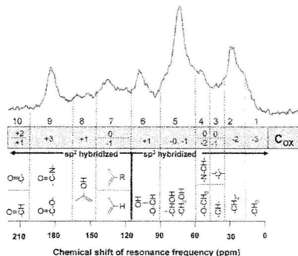
Figure 1. The direct C_{ox} assignment approach ( DD^{DA} ). Carbon ^{13}C NMR spectra are divided into 10 regions, indicated by vertical lines. Carbon functional groups in each spectral region and their corresponding resonance frequencies are shown along the lower axis. Six of the ten regions contain multiple functional groups. The horizontal dashed lines indicate additional functional group separation gained by applying a 45 \mu s dipolar dephasing delay (DD NMR).
