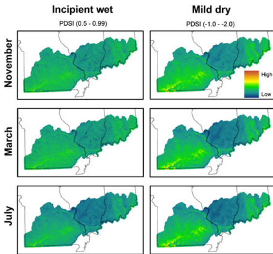
Fig. 6 Maps of fire hazard for three equally spaced months during incipient wet and mild dry conditions
