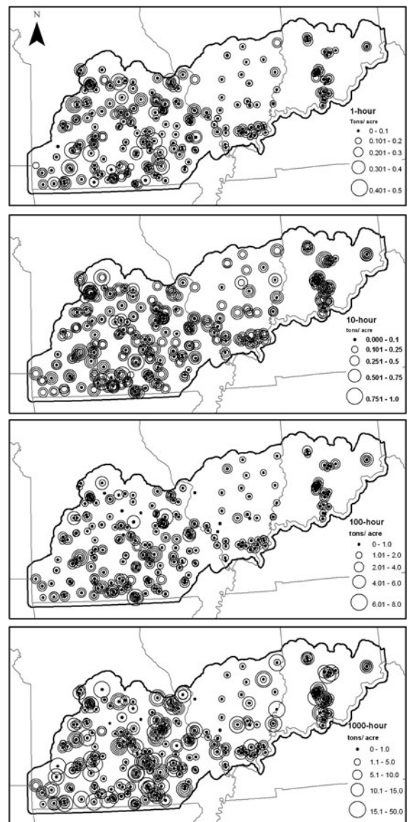
Fig. 4 Spatial patterning in fuel loading for the four time-lag fuel classes. Circle locations correspond to transect locations. Increasing circle sizes correspond to increasing fuel loading (see legend). Ranges of circle sizes represent the ranges of observed fuel loading along transects. (Convert to \text{Mg ha}^{-1} by multiplying by 2.24)
