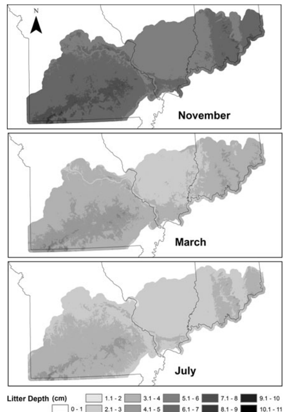
Fig. 5 Litter depth model estimates for equally spaced months during the year. Maps decrease in regional litter depth according to residence time (i.e., months since leaf fall, November)
