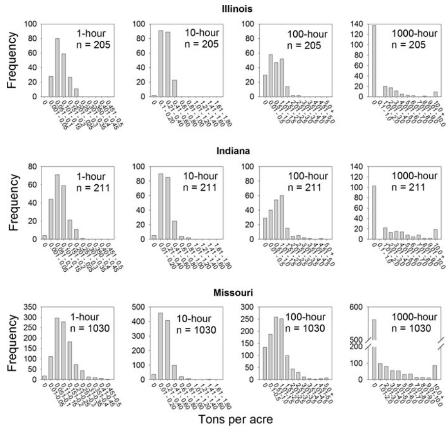
Fig. 2 Frequency distributions of fuel loading (tons \text{ac}^{-1} ) of fuels in four time-lag classes for Illinois, Indiana, and Missouri. (Convert to \text{Mg ha}^{-1} by multiplying by 2.24)
