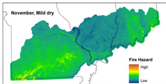
Fig. 7 Enlarged November fire hazard map. This condition represents the highest fire hazard condition predicted by the model. Fire hazard would further increase with increased drought, however less spatial complexity is expected as fuels become homogeneously dry regardless of aspect
