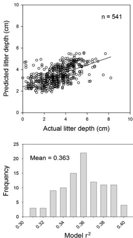
Fig. 3 (Top) Scatterplot of actual versus predicted litter depths generated from the multiple regression model (Table 2). (Bottom) Bar plot of bootstrap results of the model r -square for 100 iterations
