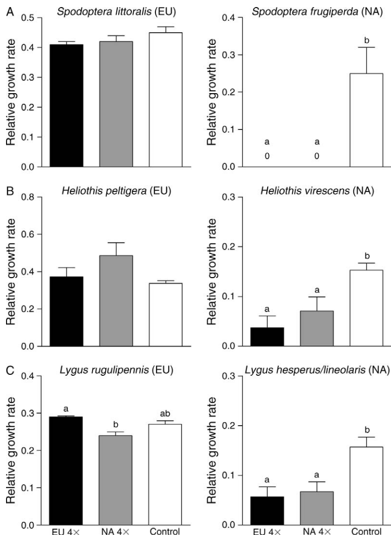
FIG. 2. Biogeographic comparisons of the relative growth rate (means \pm SE) of congenic pairs of generalist herbivores fed European tetraploid (EU 4 \times ) C. stoebe , North American tetraploid (NA 4 \times ), C. stoebe , or control plants (mixture of Pisum sativum and Lactuca sativa ). (A) Spodoptera littoralis , ANOVA, F_{2,24} = 1.039 , P > 0.2 ; Spodoptera frugiperda , Kruskal-Wallis chi = 13.310, P < 0.001 . (B) Heliothis peltigera , ANOVA, F_{2,24} = 2.514 , P > 0.05 ; Heliothis virescens , ANOVA, F_{2,31} = 9.222 , P < 0.001 . (C) Lygus rugulipennis , ANOVA, F_{2,27} = 3.360 , P < 0.05 ; Lygus hesperus/lineolaris , ANOVA, F_{2,23} = 7.135 , P < 0.01 . Different letters indicate significant differences among the plant categories (Tukey test for ANOVAs, Mann-Whitney for Kruskal-Wallis).
