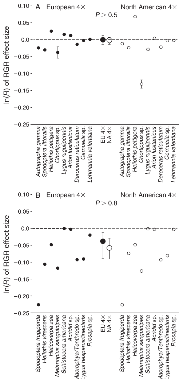
FIG. 3. Effects of European tetraploid (EU 4 \times ) and North American tetraploid (NA 4 \times ) populations of Centaurea stoebe on the relative growth rate of (A) European and (B) North American generalist herbivores. Given are the effect size measures ( e_{++} and variance) of RGR, \ln(R) , of the herbivore species tested as well as the means of the effects sizes and 95% confidence intervals separated by C. stoebe origin. Positive values indicate a relative increase in growth of herbivores on C. stoebe plants, while negative values indicate decreased relative growth rate on C. stoebe compared to controls. For the effect sizes of individual herbivores, \pm SE is either shown or smaller than the symbol. Means of effects are significant when the 95% confidence interval does not cross zero. P values test difference in effects of European vs. North American tetraploid C. stoebe .
