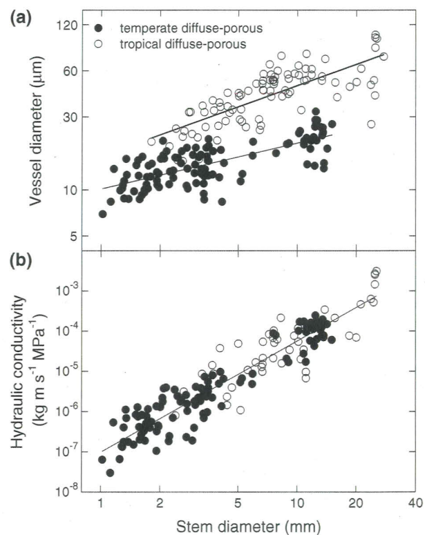
Fig. 1 Relationships between hydraulic traits and stem diameter for saplings of four temperate and four tropical diffuse-porous tree species: a vessel diameter, b hydraulic conductivity. Each data point represents an individual branch or trunk segment. Data taken from McCulloh et al. (2010)
